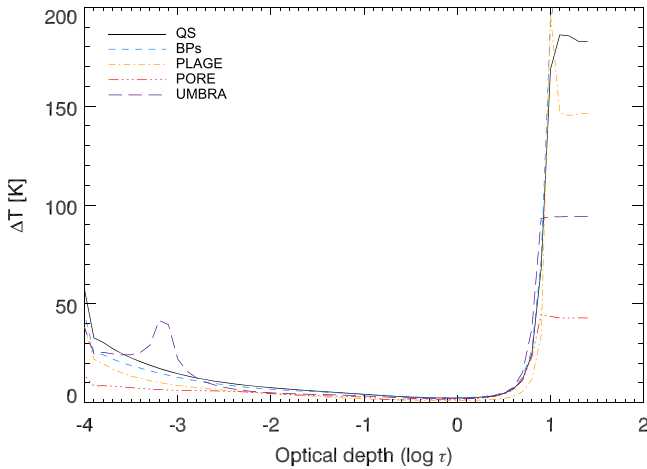
Figure 7. Temperature uncertainties for each analyzed region, as specified in the legend.
