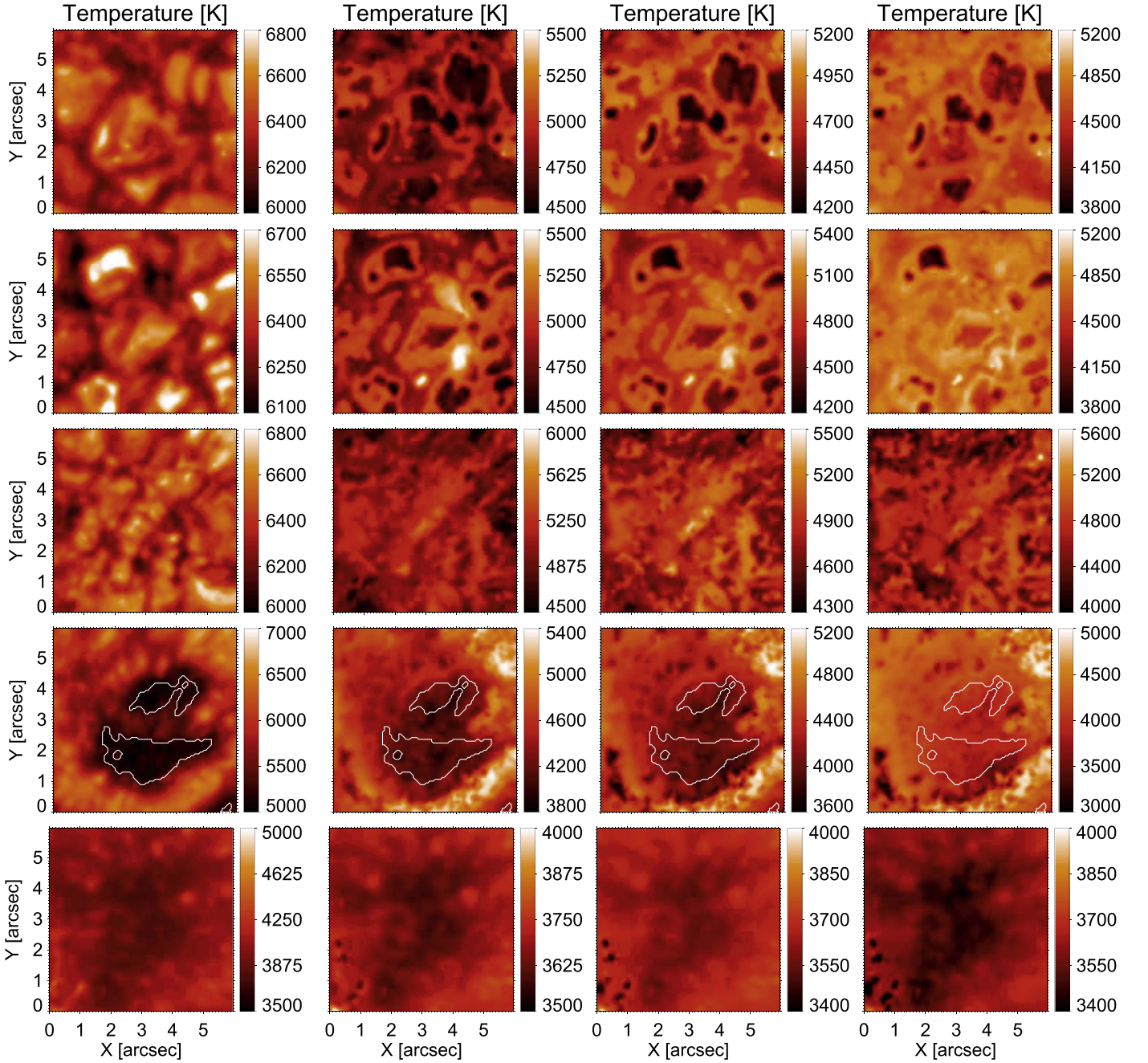
Figure 5. From left to right, top to bottom: horizontal cuts of the temperature at four different heights, specifically at \log \tau_{500} = 0, -1.5, -2, -2.5 , derived from the inversion of the QS, BPs, PL, PO, and UM data. See caption of Figure 4 for more details.
