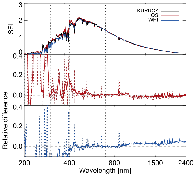
Figure 14. Top panel: SI from 200 to 2400 nm derived from our spectral synthesis performed on the QS atmosphere, calculated with the Kurucz QS model employed in the SATIRE-S model, and given by the WHI reference data considered in the NRLSSI SI model. Middle and bottom panels: relative difference between the SI derived from the synthesis on the QS atmosphere (middle) and considered in the NRLSSI model (bottom) with respect to the SI calculated with the Kurucz QS model employed in the SATIRE-S. See caption of Figure 13 for more details.
