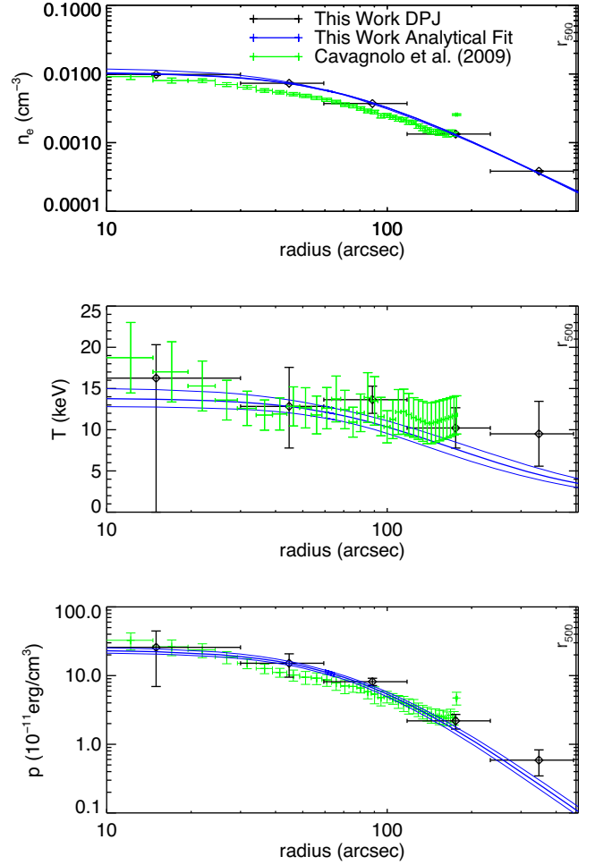
Figure B7. Abell 2219 . Our smooth parametric fit shows a decrease in temperature in the outskirts at a significance of 11.8\sigma . Jiménez-Bailón, Lozada-Muñoz & Aguerri (2013) found a shock front with >16 keV gas 2 arcmin NW of the cluster, and this elongated cluster is possibly undergoing a large merger event (Boschin et al. 2004). Further evidence for a major merger was detailed in Canning et al. (2017), who used Chandra data to identify numerous cold and shock fronts, along with a large temperature spike \sim 25 arcsec from the core of the cluster.
