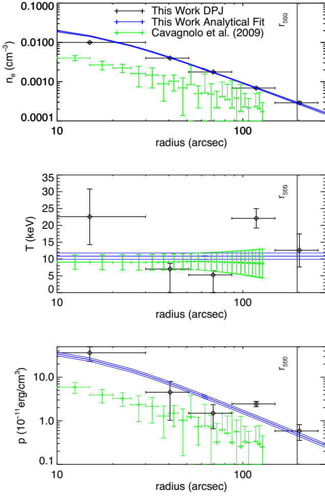
Figure B30. MACS J0257.1–2325 . The ACCEPT density profile is significantly lower compared to our and other results (Amodeo et al. 2016). Through the optical, Kartaltepe et al. (2008) found that, on large scales, this system has filaments directed into the cluster.
