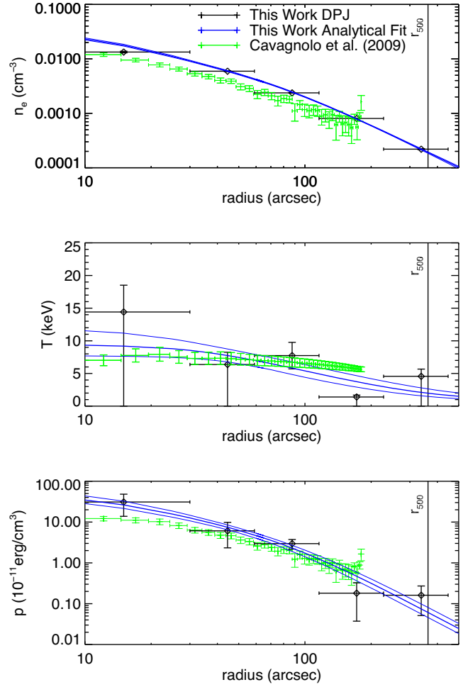
Figure B5. Abell 963. We detect a decrease in the temperature profile at large radii at a significance of 6\sigma . Our density profile is somewhat higher than that of the ACCEPT study. We do not detect the presence of a cool core, but others have found a slight temperature decrease in the centre (Baldi et al. 2007; Cavagnolo et al. 2009). Leccardi & Molendi (2008), using XMM-Newton , specifically made note of this and identified it as an ‘intermediate’ cluster since the temperature decrease in the centre is modest.
