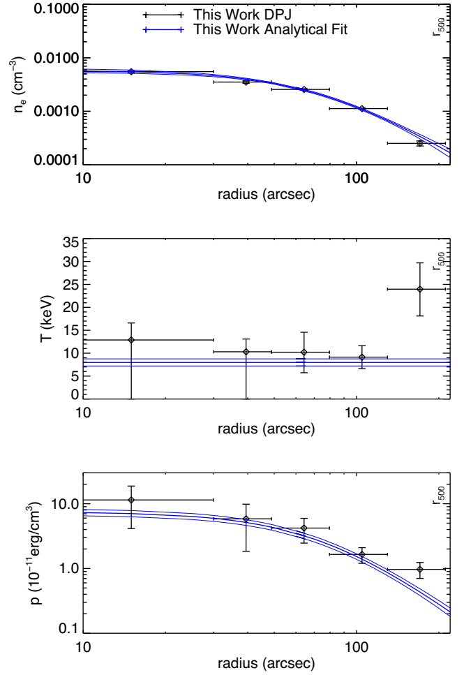
Figure B23. MACS J0416.1-2403 . Several studies have identified this cluster as a binary merger system. Mann & Ebeling (2012), using optical and X-ray data, found this system to contain a possible binary head-on collision, just after the first collision. Jauzac et al. (2015) conducted a joint X-ray and optical study, and unveiled a large structure associated with a line-of-sight filament that could not be seen in the X-ray. A large offset in the radial velocity between two subclusters was found, and their temperatures were determined to be 10 and 13.6 keV, slightly higher than our isothermal smooth parametric fit. Ogrea et al. (2015) created temperature, pressure, and entropy maps using a multiwavelength analysis of Chandra , the VLA, the GMRT, and Hubble . The temperature map is elongated, and has a relatively high mean temperature of 10 keV. The radio halo is also elongated along the same direction.
