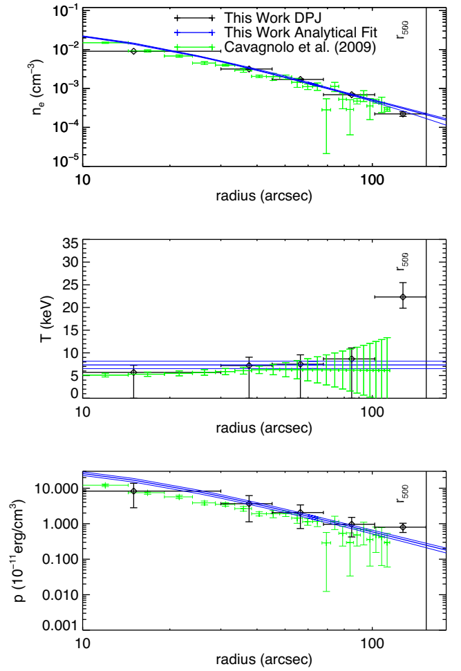
Figure B29. MACS J1311.0–0310.
