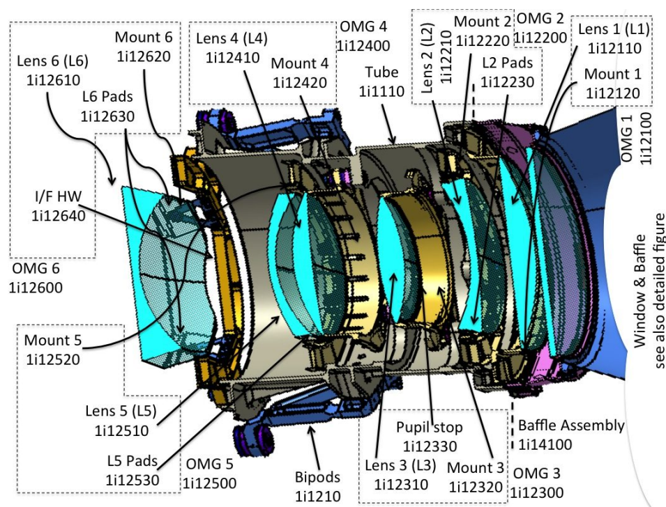
Figure 3. A cross section of the PLATO's TOU with description and coded number for several optical elements and their support. Light is getting from the right to the left and the entrance baffle is only partially shown. After a plane-parallel flat window to isolate thermally and shield from radiation the first lens, L1, provided with aspheric power, the entrance beam is defined by a physical pupil stop close to a CaF 2 lens (L3) and the beam is then converging toward the rear part of the optical train where the last element, L6, acts as a powerful field flattener onto an array of four 2500x2500 CCDs.
