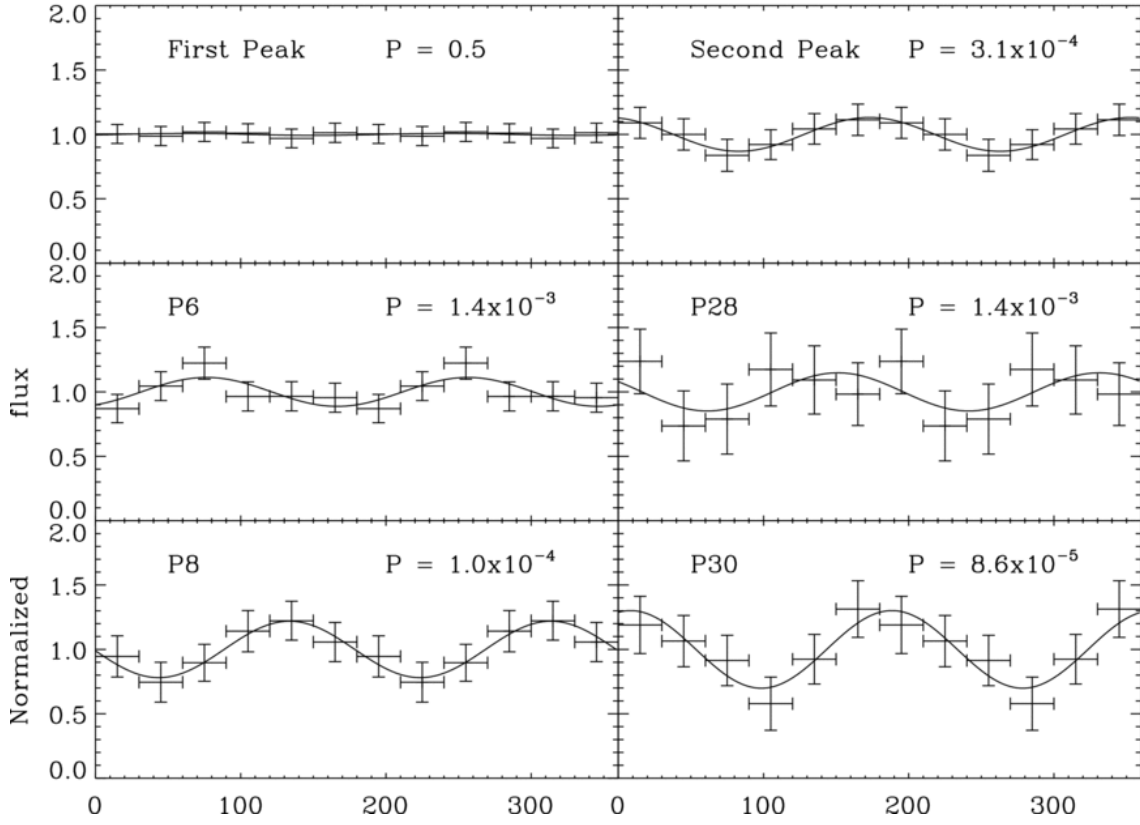
Figure 1: Polarograms of the different time intervals that have been analysed for GRB041291A (see Table 1). For comparison purposes, the curves have been normalized to their average flux level. The crosses represent the data points (replicated once for clarity) and the continuous line the fit done using Eq. 2. For each polarigram the probability, P , is shown that the polarigram measured corresponds to an un-polarized ( \Pi < 1\% ) source. From Götz et al. (2009)
