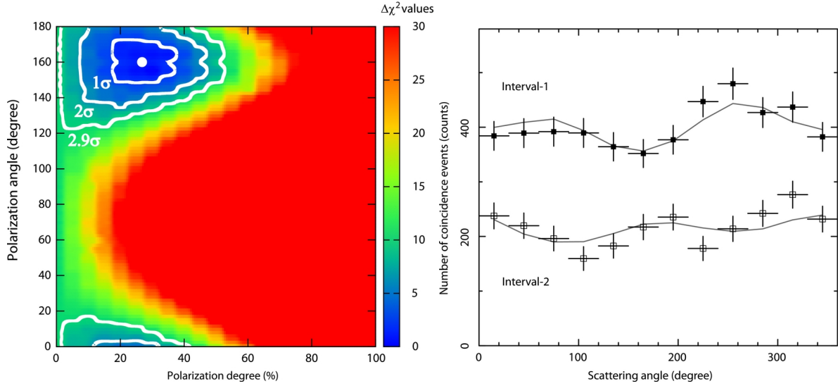
Figure 3: Left: \Delta\chi^2 map of confidence contours in the \Pi, \phi_p plane for GRB 100826A, obtained by the combined fit of the Interval-1 and -2 data. Here \phi_p is the phase angle for Interval-1. The white dot is the best-fit result, and we calculate \Delta\chi^2 values relative to this point. A color scale bar along the right side of the contour shows the levels of the \Delta\chi^2 values. The null hypothesis (zero polarization degree) can be ruled out with 99.4% ( 2.9\sigma ) confidence level. Right: Number of coincidence \gamma -ray photons (polarization signals) against the scattering angle of GRB 100826A measured by the GAP in 70–300 keV band. Black filled and open squares are the angular distributions of Compton scattered \gamma -rays of Interval-1 and -2, respectively. The gray solid lines are the best-fit models calculated with our GEANT4 Monte Carlo simulations. From (Yonetoku et al. 2011b)
