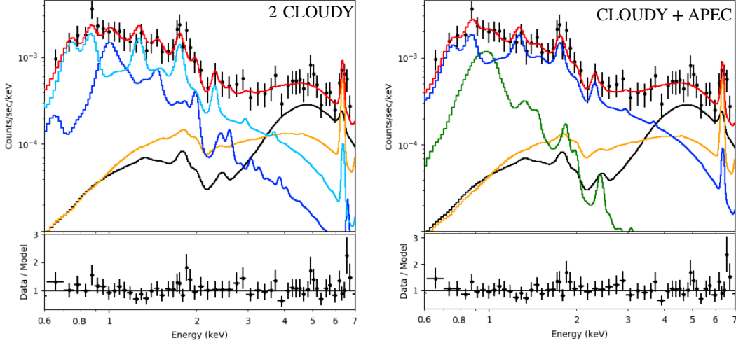
Figure 17. Spectra extracted in the NW sector, best-fit physical models and Data/Model residuals. Models consists of CLOUDY (blue, sky-blue lines), APEC (green, greenline) and PEXMON (orange) components. The black line is the nuclear spillover plus XBs spectral emission.
