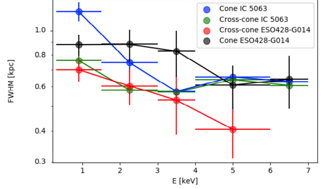
Figure 8. FWHM (units of kpc) of the radial profiles in Figs. 3 and 4 (blue, green) and for ESO428-G014 in Fabbiano et al. (2018a) (black, red) in a log space, as a function of the energy band, along the bi-cone and cross-cone direction.
