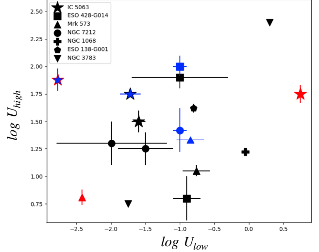
Figure 5. Lower and higher photoionization parameters of the best-fit models obtained for Seyfert galaxies in the literature, compared with our results for IC 5063 (large stars). Nuclear (black); bi-cone (blue); cross-cone (red). The blue stars show a red and a black edge indicating the values for the NW and SE cone, respectively. The blue marks by ESO428-G014 (Fabbiano et al. 2018a) and NGC 7212 (Jones et al. 2020) represent values obtained from the spectral fits in the extended annular region, where, however, the emission along the cones dominates. We included the following Seyferts: Mrk 573 (Paggi et al. 2012), NGC 1068 (Kraemer et al. 2015), ESO-138-G001 (De Cicco et al. 2015) and NGC 3783 (Kaspi et al. 2002; Blustin et al. 2002).
