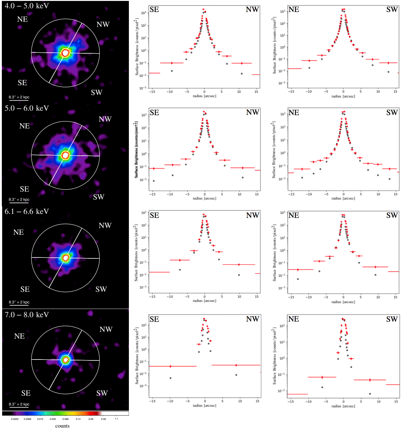
Figure 4. Top panels: 4.0-5.0 keV, top/middle panels: 5.0-6.0 keV, bottom/middle panels: 6.1-6.6 keV, bottom panels: 7.0-8.0 keV. See caption in the Fig. 3 for details.
