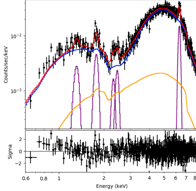
Figure 11. Leaky Absorber fit to the nuclear spectrum of IC 5063 (top panel) and residuals (bottom panel). The spectrum is extracted from a circle of 2'' radius ( \sim 3\text{--}4 PSF) and binned at 20 counts per bin. The total model (red line) includes a partially absorbed power law (blue line), a PEXRAV reflection component (orange line) and five Gaussian lines (purple lines).
