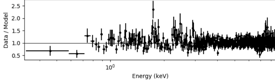
Figure 14. Residuals (data/model) obtained by fitting the nuclear spectrum with a single CLOUDY model.
