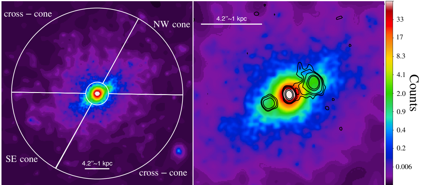
Figure 2. Left panel reports the adaptively smoothed (similarly to the images in Fig. 1), 1/8 pixel image of the emission at the 0.3-7.0 keV band. White full lines divide the nucleus of IC 5063 from the extended ( >2'' ) region which, in turn, is split in four regions with opening angles of \approx 60 and 120^\circ , to separate the bi-cone from the cross-cone area. Specifically, the bi-cone regions are enclosed in North-West (NW) and South-East (SE) sectors and limited at the position angles 269^\circ - 331^\circ and 89^\circ - 151^\circ , respectively. In the right panel, we show the zoom-in of the IC 5063 nucleus. Black contours represent the radio emission observed with ATCA at 17 GHz and levels 3,5,10,50,100 \sigma ( \sigma \approx 0.11 mJy beam ^{-1} ; Morganti et al. 2007).
