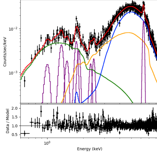
Figure 12. Soft excess power law to fit the nuclear spectrum (top panel) and residuals (bottom panel). The soft ( <2 keV) X-ray emission is fitted with a unabsorbed power law component with \Gamma=2.2 (green line) plus eight Gaussian emission lines. The hard ( >2 keV) X-ray spectral fit consists of a Gaussian emission line, to model the Fe-K \alpha transition, and an highly obscured power law (blue line) and an intrinsically absorbed reflection PEXRAV (orange line) with \Gamma=1.7 and neutral hydrogen column density N_H \sim 3.5 \times 10^{23} \text{ cm}^{-2} and N_H \sim 3.1 \times 10^{22} \text{ cm}^{-2} , respectively.
