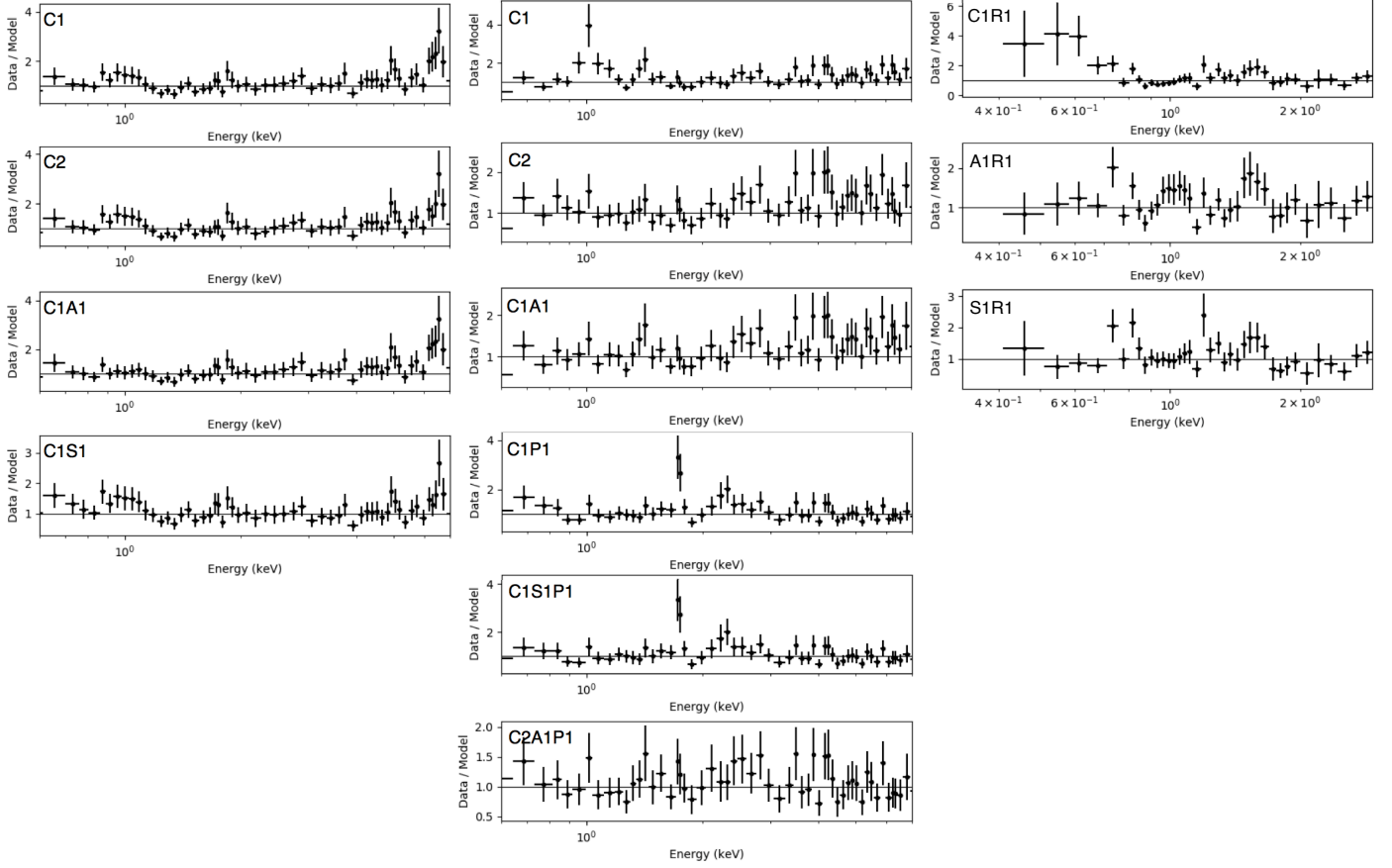
Figure 20. Residuals (data/model) obtained by fitting the NW (left), SE (center) cone and cross-cone (right) spectra with intermediate models used in the procedure described in Sect. B.3. Models represent a combination of CLOUDY (C), APEC (A), PSHOCK (S), PEXMON (P) and PEXRAV (R) templates.
