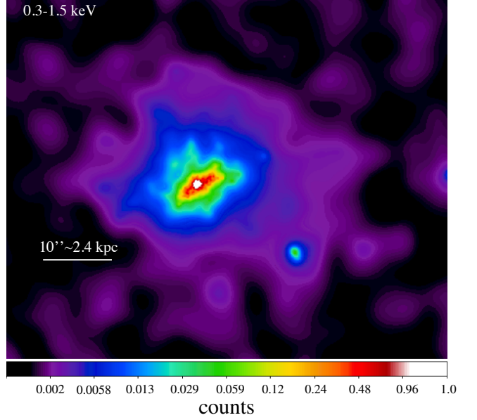
Figure 7. 0.3-1.5 keV image, adaptively smoothed with Gaussian kernels ranging from 0.5 to 30 image pixel (1/8 of instrumental pixel) in 30 iterations and 10 counts under the kernel. The color bar is in counts per image 1/8 subpixel.
