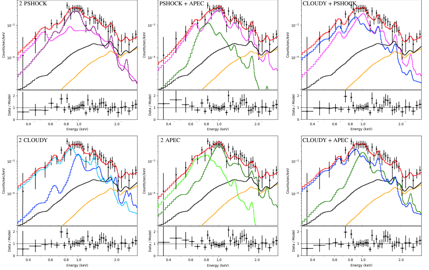
Figure 19. Soft (0.3-3 keV) X-ray spectrum extracted in the cross-cone sectors, best-fit physical models (red lines) and Data/Model residuals. Models consists of CLOUDY (blue, sky-blue lines), APEC (green, greenlime) and PSHOCK (magenta, purple lines) components. The black and orange lines are the nuclear spillover plus X-ray binaries spectral emission and the PEXRAV reflection component, respectively.
