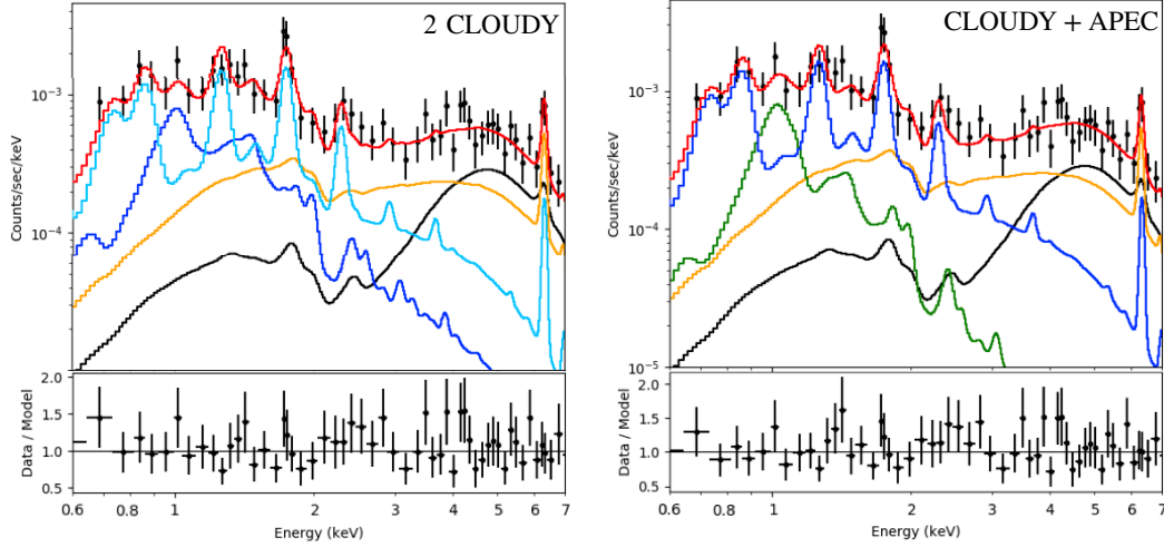
Figure 18. Spectra extracted in the SE sector, best-fit physical models and Data/Model residuals. Models consists of CLOUDY (blue, sky-blue lines), APEC (green, greenline) and PEXMON (orange) components. The black line is the nuclear spillover plus XBs spectral emission.
