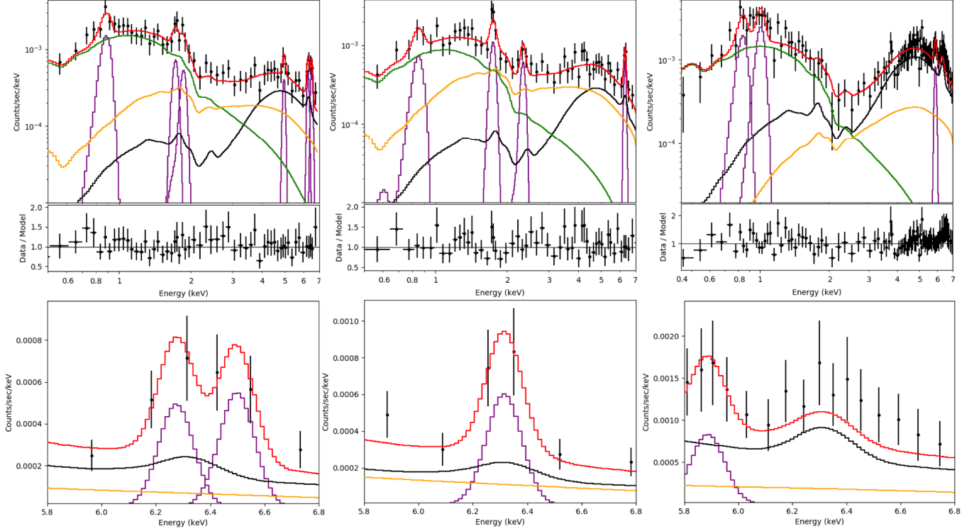
Figure 15. Top panels: spectra extracted from the NW cone (left), SE cone (center) and cross-cone (right) sectors and binned at 20 counts per bin. For each we report the best-fit empirical model and residuals. Models consists of a power law component (green), a Compton reflection PEXRAV component (orange) and some emission lines (purple). The black lines are fixed templates representing a spectral model due to the nuclear spillover plus X-ray binaries emission we derive in Sect. B.1. Bottom panels: Zoom-in of the iron transitions in the spectral region 5.8-6.8 keV of the spectra above.
