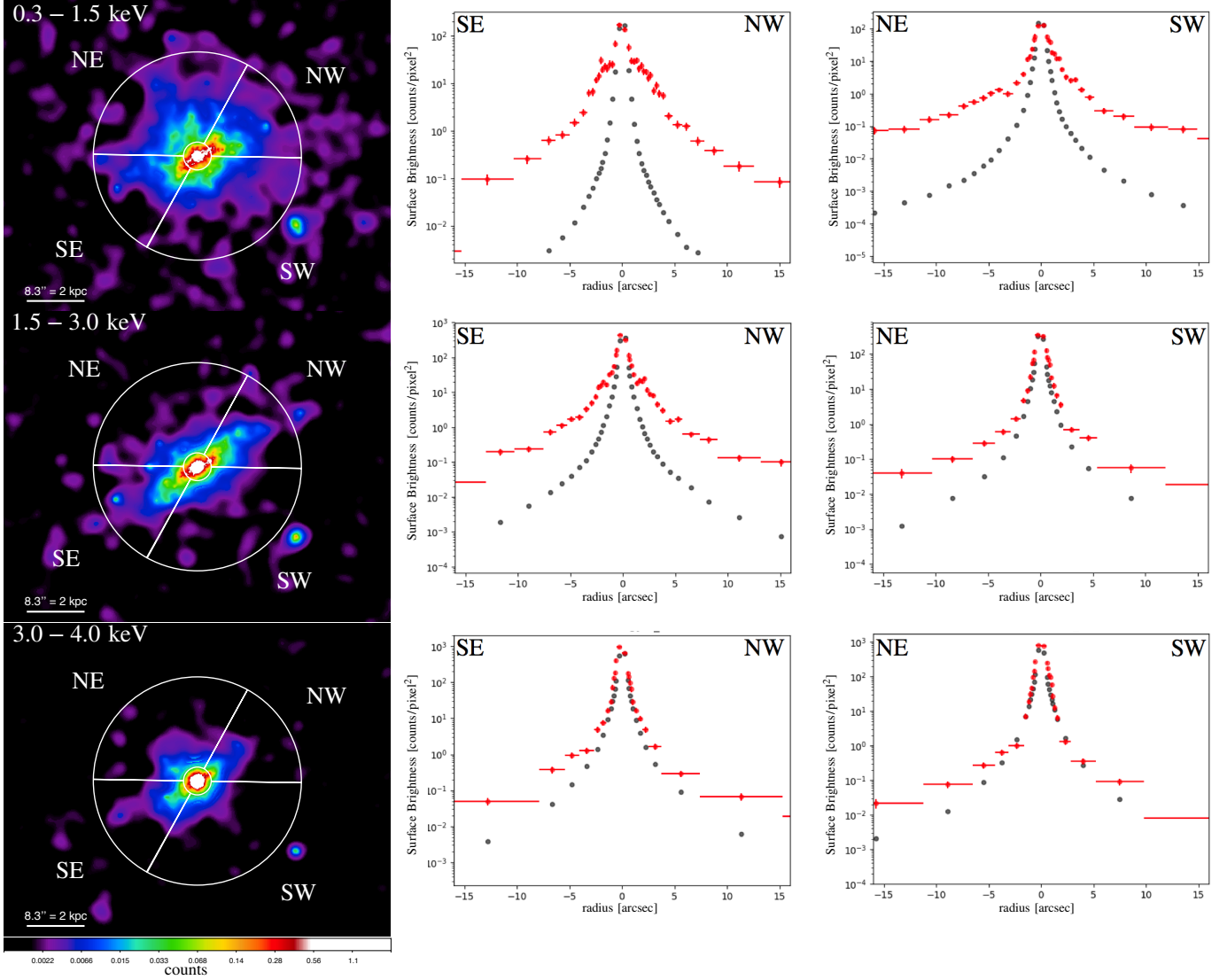
Figure 3. Images (left column) and surface brightness radial profiles in the bi-cone (central column) and cross-cone (right column) sectors, of IC 5063 in different energy bands ( top panels : 0.3–1.5 keV, middle panels : 1.5–3.0 keV, bottom panels : 3.0–4.0 keV). The images are re-binned at 1/8 of native pixel and adaptively smoothed with dmimgadapt (setting the following parameters: min=1 , max=15 , num=12 , radscale=log , counts=5 ). The radial profiles are background-subtracted and estimated from the 1/8 sub-pixel images (red) and from the normalized PSF-model images (black). Uncertainties are 1\sigma and the bin size was chosen to contain a minimum of 25 counts.
