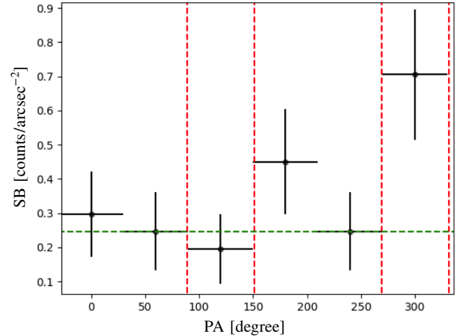
Figure 10. Surface brightness (in counts/arcsec 2 ) azimuthal profile within the 432-840 pc annulus (white annulus in Fig. 9) in the 6.5-6.8 keV image, used as a proxy of the ionized iron line. Red dashed lines separate the bi-cone and cross-cone sectors we consider throughout the paper, while green dashed horizontal line is the average surface brightness estimated excluding the two peak values at 120^\circ and 300^\circ .
