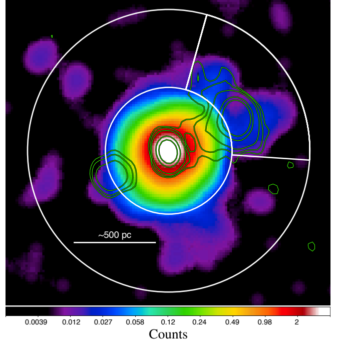
Figure 9. Merged 6.5-6.8 keV image with 1/8 of the ACIS pixel and a Gaussian smoothing with a 10 sub-pixel kernel radius, as a proxy of the ionized iron emission line morphology. In white, we report both the 1.8'' to 3.5'' annulus, and the NW cone sector in which we detect the ionized iron feature at \sim 6.6 keV from the spectral analysis. In green we overlap radio emission contours at 17 GHz and levels 3, 5, 10, 50, 100\sigma (see Fig. 2).
