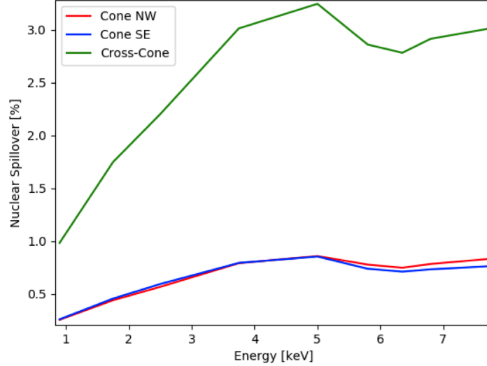
Figure 16. Contribution (in %) of the nuclear spillover in the different extended regions as a function of the energy.
