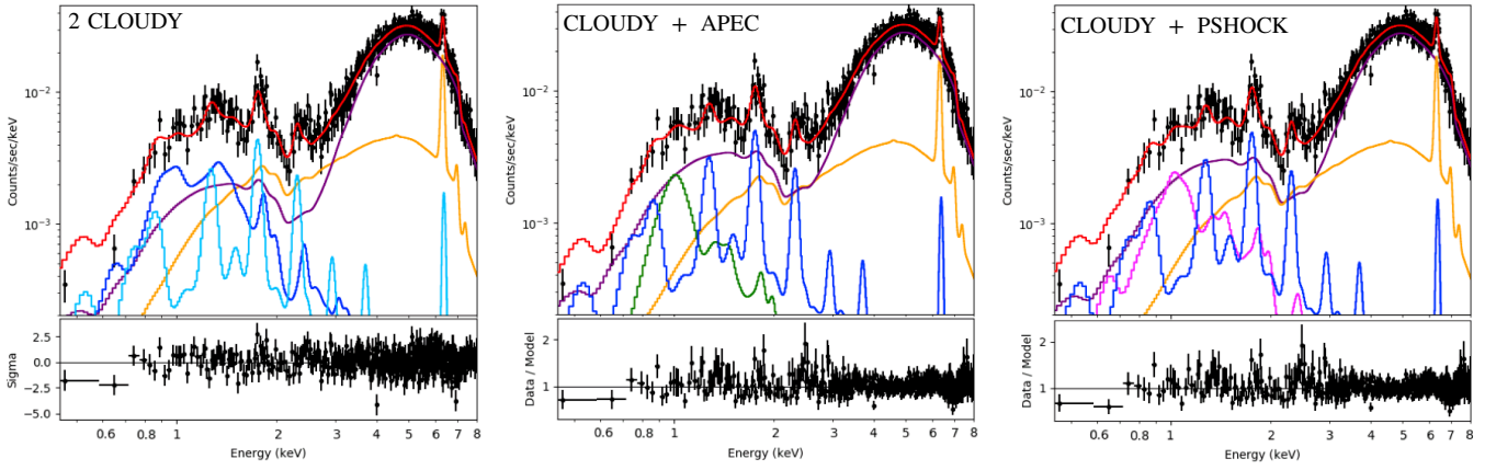
Figure 13. Best-fit physical models and residuals for the nuclear spectrum. Spectral fit consists of a leaky absorber model (purple), a PEXMON reflection component (orange), plus a mix of photoionization CLOUDY (blue and sky-blue), collisional plasma APEC (green) and shock PSHOCK (magenta) models.
