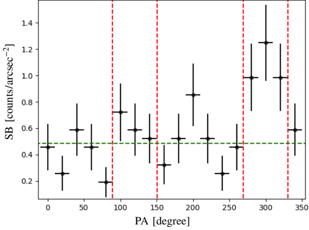
Figure 6. Surface brightness (in counts/arcsec 2 ) azimuthal profile from 0.5 to 1.2 kpc in the 6.1-6.6 keV image (Fe K \alpha ). Red dashed vertical lines separate the bi-cone and cross-cone sectors, and the green dashed line indicates the average of the surface brightness, which is estimated excluding the points in the NW sector.
