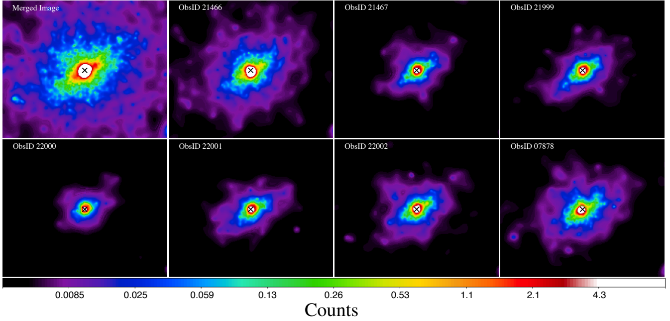
Figure 1. Adaptively smoothed (using dmimgadapt ; see text for details), 1/8 sub-pixel images of the all observations plus the final merged image (top-left first), which is obtained by aligning all seven images. N is up and E to the left. In each image we report a black cross indicating the counts peak position used to align the sub-array mode observations, and we identify the data from which the image was derived. The only full-array mode observation, i.e. ObsID 7878, is aligned by matching the X-ray point sources in the field with respect to the deepest observation, i.e. the ObsID 21466 (see text for details).
