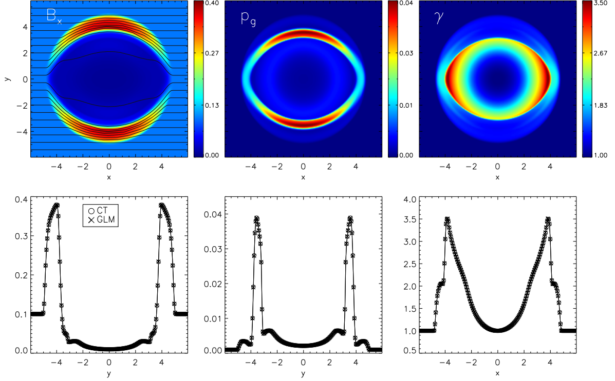
Figure 6. Cylindrical explosion at t = 4 using \eta = 10^{-6} . Upper panels show, from left to right, the x -component of magnetic field, gas pressure, and Lorentz factor computed using the CT scheme and the MHLIC Riemann solver. In the lower panels, we plot the corresponding profiles along the y -axis (for B_x and p_g ) or the x -axis (for the Lorentz factor). Results obtained with the CT and GLM schemes are shown using circles and \times symbols.
