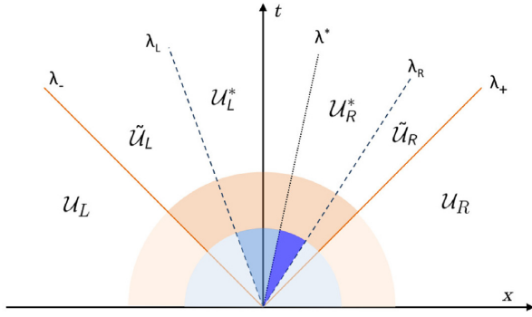
Figure 3. Schematic representation of the Riemann fan assumed by the MHLIC solver. The outermost waves ( \lambda_+ = -\lambda_- = 1 ) are EM (light) waves, while \lambda_L and \lambda_R are pairs of acoustic waves. The central mode ( \lambda^* ) represents a contact discontinuity. Jumps in EM fields are denoted by different shades of orange, while jumps of hydrodynamic variables are marked by different shades of blue.
