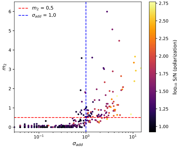
Figure 7. Comparison of the \sigma_{\text{add}} and m_2 complexity metrics for polarized components in the median-filtered GL observation. The points are colored by \log_{10}(\text{S/N}_{\text{pol}}) , and the thresholds for complexity for both metrics are shown by dashed lines: \sigma_{\text{add}} = 1 (blue vertical) and m_2 = 0.5 (red horizontal). Note that the \sigma_{\text{add}} axis is on a log scale, while the m_2 axis is on a linear scale.
