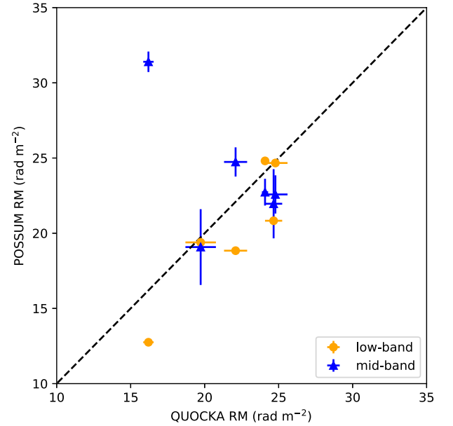
Figure 9. Comparison of EL and EM POSSUM RMs to RMs from the QUOCKA survey. POSSUM EL RMs are plotted as orange circles, and POSSUM EM RMs are plotted as blue triangles.
