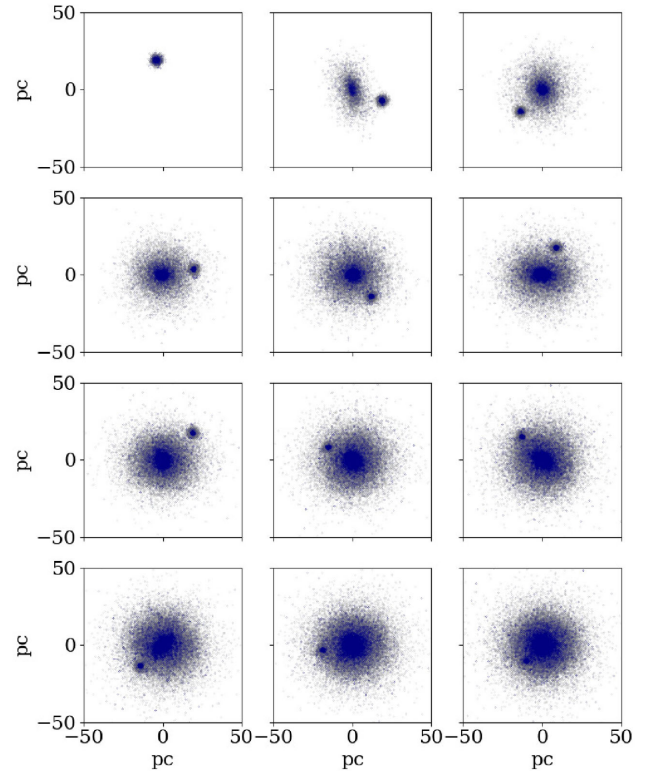
Figure 2. Snapshots of the spatial distribution of the neutron stars (blue dots) in the NSC on top the background stellar component (grey dots). Each snapshot is taken when a new globular cluster is injected in the simulation.
