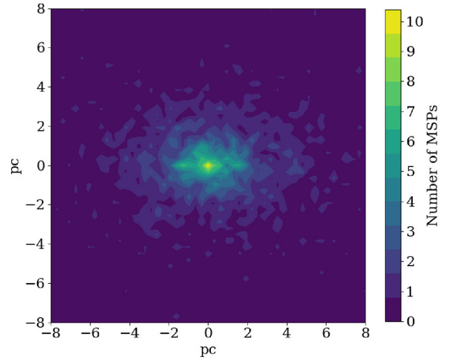
Figure 6. Colour-scale map of the distribution of the MSPs at the Galactic Centre. The map is built on a grid of pixels size \sim 0.32 pc, which corresponds to the telescope beam for Case 1 and Case 2.
