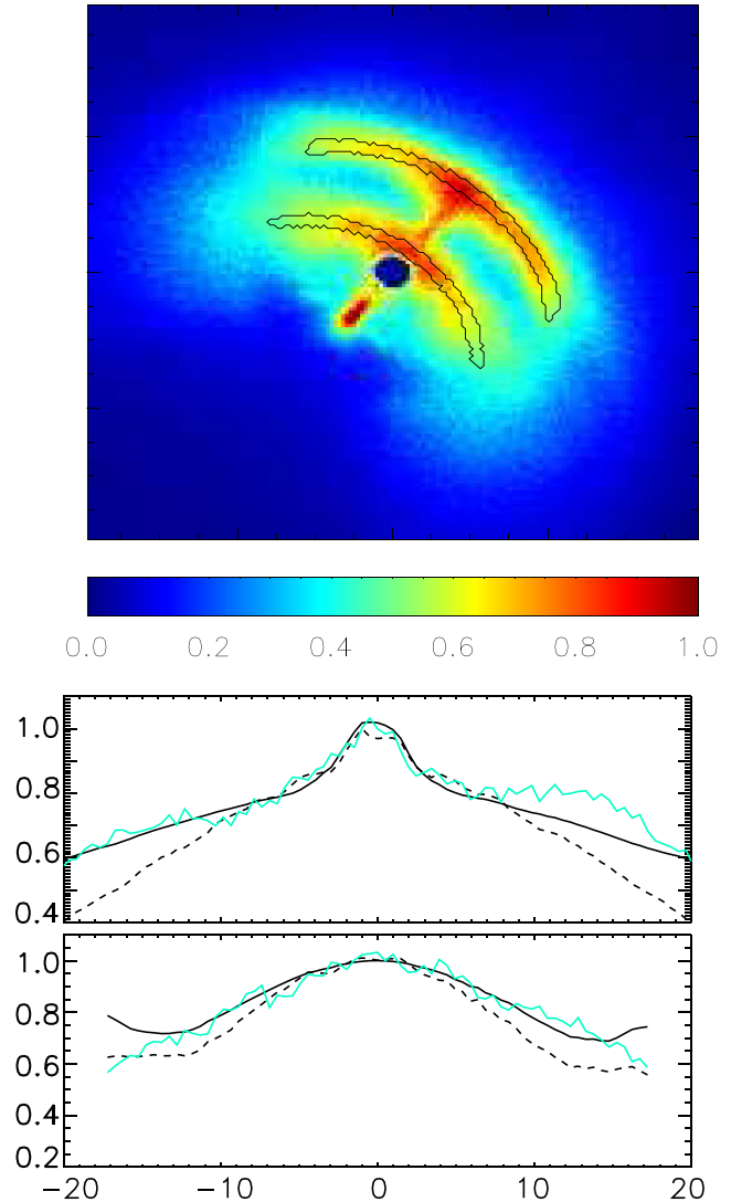
Figure 6. Upper panel: brightness map of the Vela PWN, normalized to the maximum. Axes in arcsecs. The central region containing the pulsar has been excised. The two arcs represent the region of the inner torus and outer torus whence the brightness profile was extracted. Lower panel: comparison of the surface brightness in the outer torus (above) and inner torus (below), measured in the arcs shown in the upper panel, to the model with \sigma = 1 (solid line) and to the one with \sigma = 0 (dashed line). The x-axis is in arcsec from the peak. The y-axis is in arbitrary units normalized to the peak.
