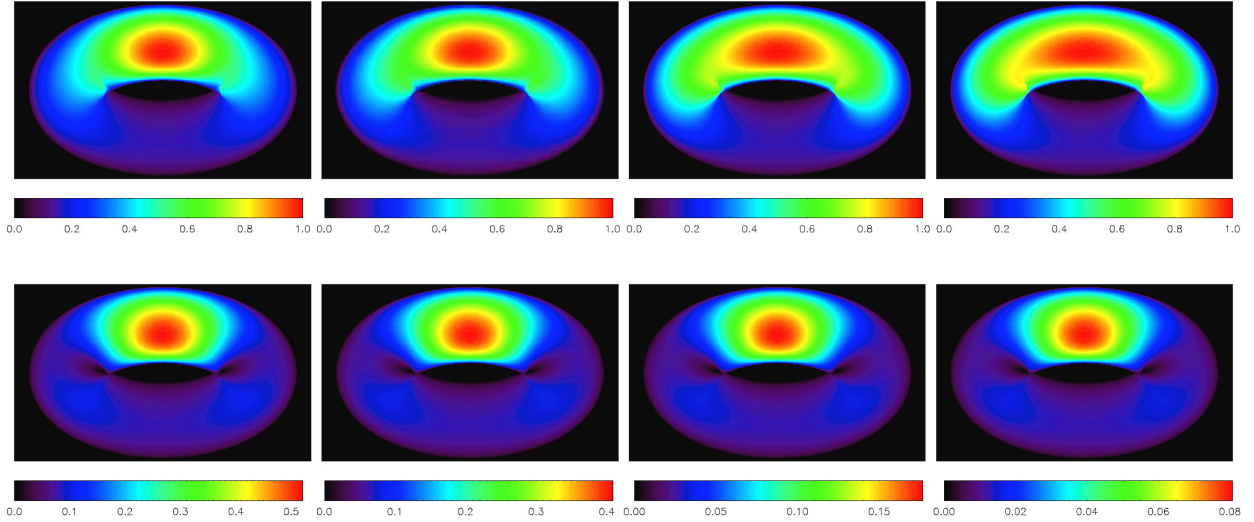
Figure 1. Upper panels: from left to right the total intensity normalized to its maximum value, for \sigma = \sqrt{1/6}, \sqrt{1/3}, \sqrt{4/3}, \sqrt{10/3} (corresponding to ratios of energy in the fluctuating components over the one in the ordered toroidal component of 0.5, 1, 4, 10, respectively). Lower panels: the same but for the polarized intensity, normalized to the maximum total intensity.
