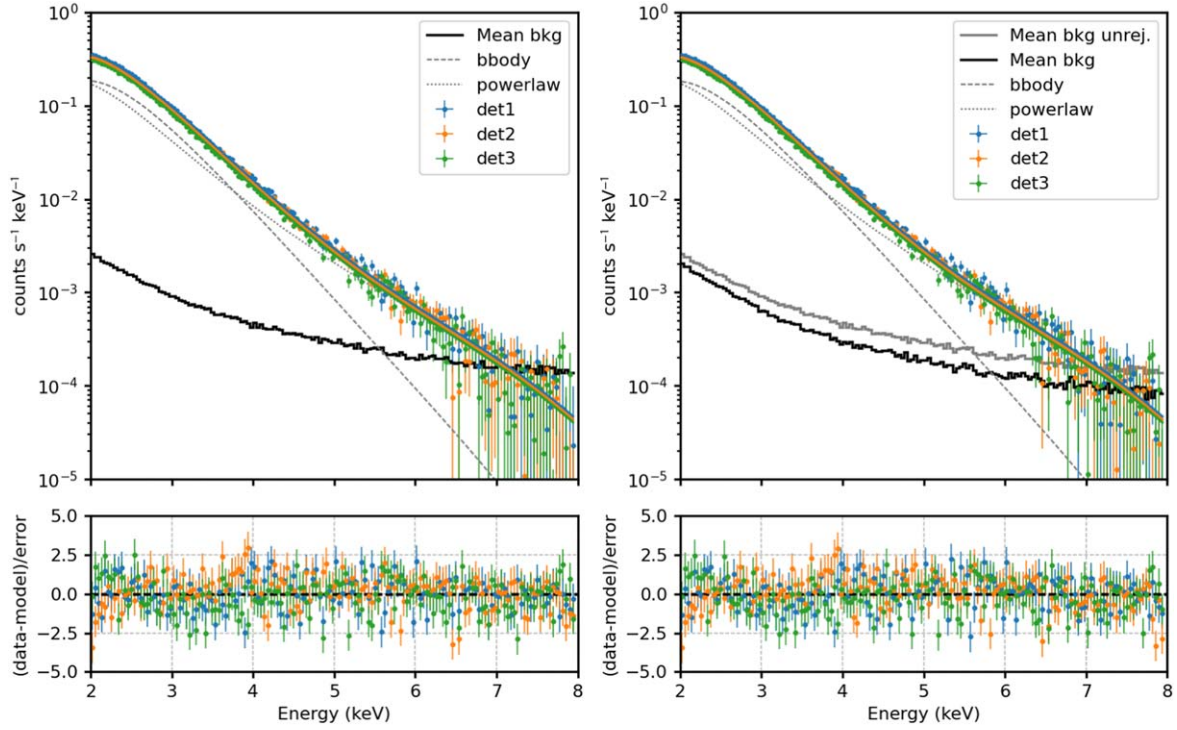
Figure 19. 4U 0142+61 data fitted with XSPEC before (left) and after (right) the background rejection; the considered spectral model is TBABS*(BBODY+POWERLAW). At the bottom, residuals with respect to the best-fit model are shown. On the right panel, the backgrounds before and after rejection are compared, and it is possible to appreciate its reduction after the rejection procedure.
