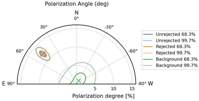
Figure 18. Contours enclosing regions at the confidence level of 68.3% (solid lines) and 99.7% (dotted lines) in case of original unrejected data (light blue), after the rejection of Section 4.2.4 (orange) and for the events rejected because identified as background (green).
