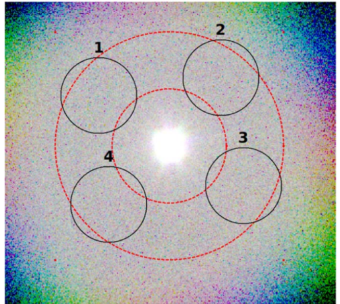
Figure 3. IXPE observation of 4U 0142+61 overimposed with four circular regions, in black, with radius 100'' and an annular region, dotted line in red, with inner radius 2.5' and outer radius 5' . These regions are used to test and compare different background selections in this analysis.
