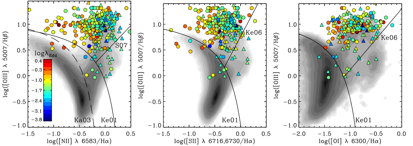
Figure 1. Emission-line diagnostic diagrams for the BASS sources with signal-to-noise ratio ( S/N ) > 3 . Left-hand panel: [N II] \lambda 6583/\text{H}\alpha versus [O III] \lambda 5007/\text{H}\beta diagnostic diagram. Colour filled circles and triangles indicate type 1 AGN (including type 1.9) and type 2 AGN, respectively. The empirical star formation curve obtained from Kauffmann et al. (2003) (dashed curve) and the theoretical maximum starburst model of Kewley et al. (2001) (solid curve) are used. The solid straight line is the empirical demarcation of Schawinski et al. (2007) distinguishing the Seyfert AGN from the LINERs. The Eddington ratio of BASS sources is shown with colour-filled dots. Middle panel: [S II] \lambda\lambda 6716, 6731/\text{H}\alpha versus [O III] \lambda 5007/\text{H}\beta diagnostic diagram. Right-hand panel: [O I] \lambda 6300/\text{H}\alpha versus [O III] \lambda 5007/\text{H}\beta diagnostic diagram. Demarcation lines from Kewley et al. (2001, 2006) are used. In all panels, we also show more than 180 000 SDSS emission-line galaxies with filled contours chosen from the OSSY catalogue ( z < 0.2 ) with S/N > 3 for [N II] \lambda 6583 , H \alpha , [O III] \lambda 5007 , H \beta , [S II] \lambda 6716 , [S II] \lambda 6731 , and [O I] \lambda 6300 .
