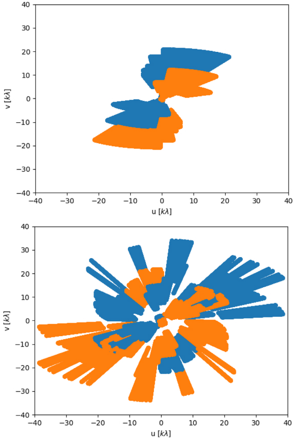
Figure 1. A 1300 (top panel) and MACS J1931.8–2634 (bottom panel) uv coverages over the entire bandwidth. Only 1 out of every 10 points in time and 1 out of every 40 points in frequency are plotted. The two colours show the symmetric uv points obtained from the conjugate visibilities. Note that the different uv coverage for the two clusters reflects into a different synthesized beam (Table 1).
