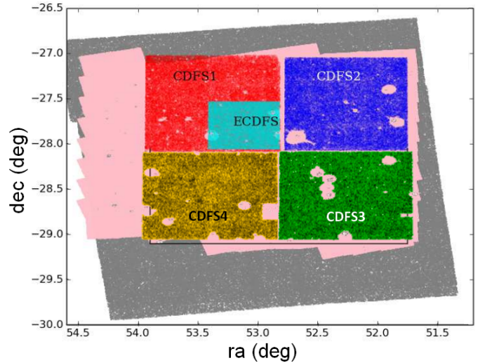
Fig. 1. Chandra Deep Field South as imaged by different surveys (gray: SWIRE, pink: SERVS, cyan: ECDFS, other colors: VST-CDF-S regions). Adapted from Falocco et al. (2015).
