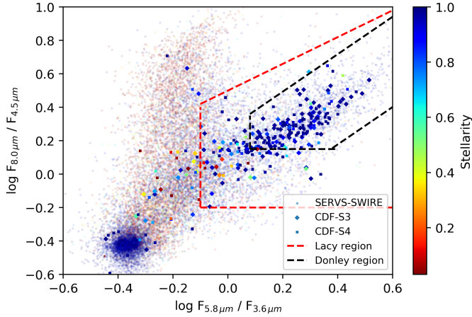
Fig. 8. Mid-infrared diagnostic by Lacy et al. (2004, 2007). Dots: SERV-SWIRE reference population. Diamonds: CDF-S3 variable sources. Squares: CDF-S4 variable sources. Color bar: stellarity index from 0 (red) for galaxies to 1 (blue) for star-like sources. Red dashed lines: Lacy et al. (2007) AGN selection criteria. Black dashed lines: Donley et al. (2012) AGN selection criteria.
