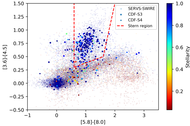
Fig. 9. Mid-infrared diagnostic proposed by Stern et al. (2005). Dots: SERV-SWIRE reference population. Diamonds: CDF-S3 variable sources. Squares: CDF-S4 variable sources. Color bar: stellarity index from 0 (red) for galaxies to 1 (blue) for star-like sources. Red dashed lines: Stern et al. (2005) AGN selection criteria.
