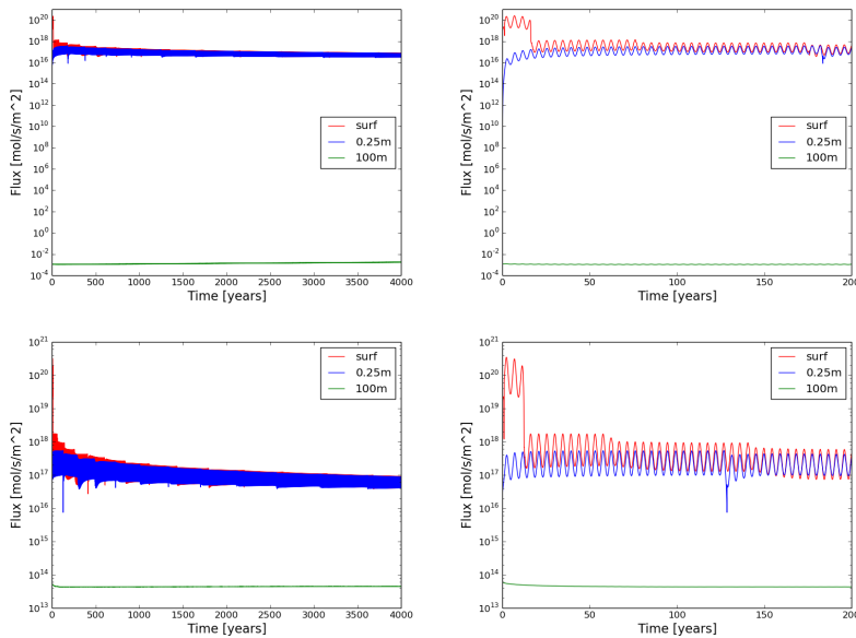
Fig.2: Water flux vs time at the equator for initial temperature of 80 K (on the top) and 163 K (on the bottom) for porosity of 0.6.
