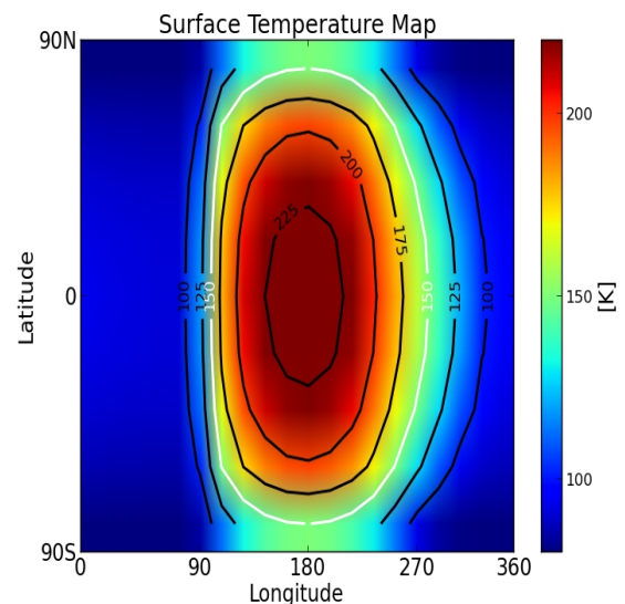
Fig.1: Typical surface temperature.
