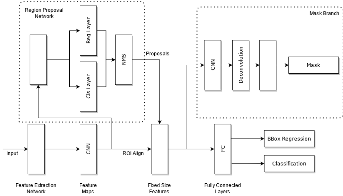
Fig. 3. Mask R-CNN architecture.
