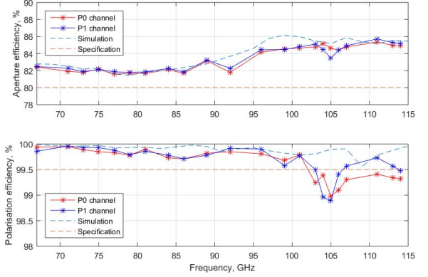
Fig. 4. Comparison between the measured and simulated aperture and polarization efficiencies for the UdC horn, including the lens, followed by INAF OMT. Aperture efficiencies are fully compliant to ALMA specification of >80\% across full frequency range. Polarization efficiencies are mostly compliant to ALMA specification of >99.5\% , with some degradation above 101 GHz.
