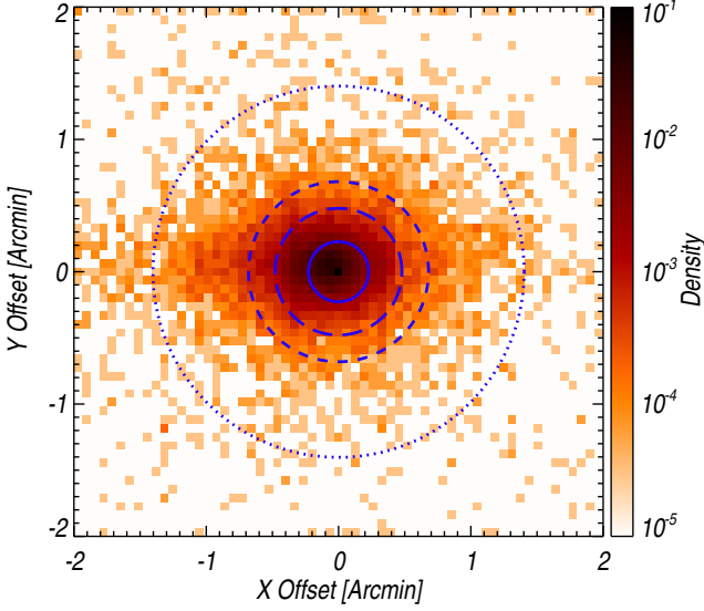
Fig. 5. Density distribution of the positional offsets computed from 100 000 Monte Carlo realizations. Circles show the cumulative distributions at 68% (solid line), 90% (long-dashed line), 95% (dashed line) and 99% (dotted line).
