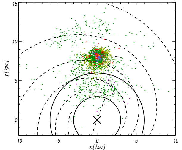
Fig. 10. Distribution of the PGCC sources as seen from the North Galactic pole. Only distance estimates with a DIST_QUALITY flag equal 1 and 2 are plotted. Different methods have been used to derive the distances: kinematic (purple), optical extinction (blue), near-infrared extinction (green), molecular complex association (orange), and Herschel HKP-GCC (red). We also show the distribution of the distance upper-limits (DIST_QUALITY=4) provided by the near-infrared extinction method (light green). The red dashed circle shows the 1 kpc radius around the Sun. Black dashed lines represent the spiral arms and the local bar. The black circles, centred on the cross, provide an indication of the location of the molecular ring.
