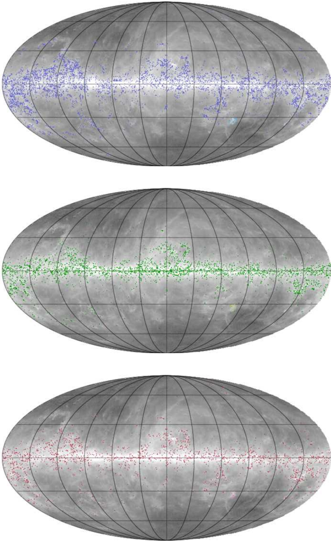
Fig. 2. All-sky distribution of the PGCC sources according to their FLUX_QUALITY category: "Reliable flux densities" (FQ=1, top panel), "Missing 3 THz flux density" (FQ=2, middle panel) and "Detection only" (FQ=3, bottom panel). Sources located in the LMC and SMC are also shown in light colours.
