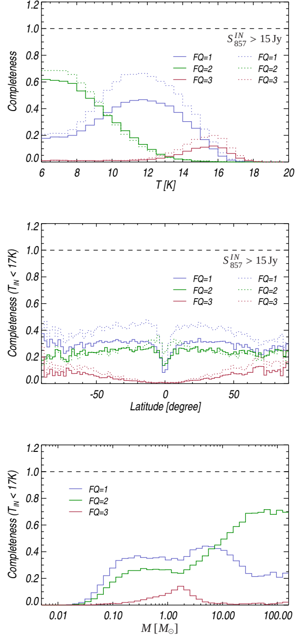
Fig. 3. Completeness as a function of the input temperature ( top panel ), latitude ( middle panel ), and mass ( bottom panel ) of the injected sources. For the latitude and mass cases, the input temperature was lower than 17 K. In addition, when considering the dependence of completeness on mass, all the sources are assumed to be at 100 pc from the Sun. Each panel shows the distributions obtained from selecting only the sources in a given FLUX_QUALITY category. In particular, FQ=1, 2 and 3 correspond to the blue, green and pink curves, respectively. Finally, the dotted line in each panel denotes the completeness for the sample of sources with input flux density S_{857}^{IN} > 15 Jy.
