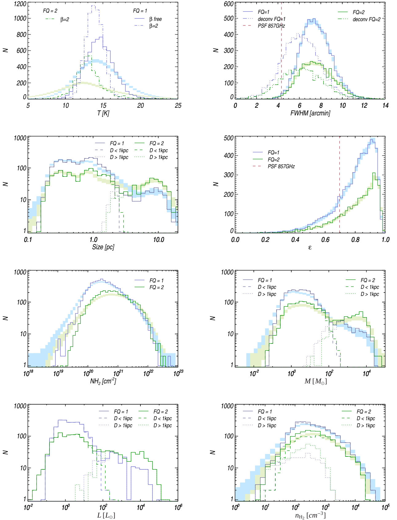
Fig. 11. Distribution of the physical properties of the PGCC objects with FQ=1 (blue) and FQ=2 (green). The coloured shaded regions provide an estimate of the impact of the individual uncertainties on the statistical distribution at a 1\sigma dispersion level around the mean value obtained from 10 000 MC realizations (see Sect. 6 for more details). The temperature distribution is shown for two temperature estimates, i.e., using a free emissivity spectral index \beta (solid line) or a fixed \beta=2 (dot-dashed line). The distribution of the intrinsic size, after deconvolution, is shown on the top right panel in dot-dot-dot-dashed line. The distributions of the physical size, mass, mean density and luminosity of the clumps are provided for sources with reliable distance estimates (DIST_QUALITY=1 or 2). These distributions are also shown separately for sources at solar distances smaller or larger than 1 kpc from the Sun, in dashed and dotted lines, respectively.
