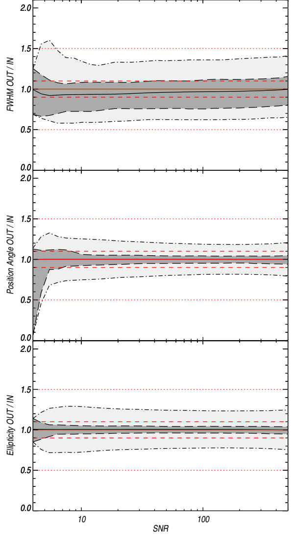
Fig. 6. Ratio of the recovered (OUT) to injected (IN) geometric parameters for the simulated sources detected with FQ=1 and 2 : \theta ( top ), position angle ( middle ) and ellipticity ( bottom ). The ratio is given as a function of the detection S/N estimated from the cold residual maps. The light and dark grey shaded regions (denoted by the dot-dashed and long-dashed lines, respectively) highlight the behaviour of 95% and 68% of the sources, respectively, in each S/N bin. The median of the ratio distributions are shown with a solid line. The 0%, 10% and 50% levels of uncertainty are overlaid using a red solid, dashed and dotted line, respectively.
