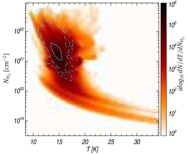
Fig. 14. Temperature vs. column density two-dimensional distribution for all PGCC cold clumps followed-up by Herschel in the HKP-GCC programme. The plotted data points are identified as IN and OUT: IN points are located inside the Planck clump solid angle, while the OUT points are located outside. The distribution of the OUT points is shown in colour, while the distribution of the IN points is denoted by cyan contours at three different levels: 10, 50 and 90% of the maximum.
