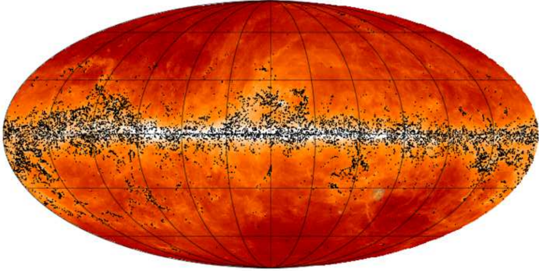
Fig. 1. All-sky distribution of the PGCC sources: 13188 Galactic clumps ( black dots ), plus 54 Large Magellanic Cloud (LMC) and Small Magellanic Cloud (SMC) clumps ( grey dots ). The source distribution is overlaid on the 857 GHz Planck map, shown in logarithmic scale between 10^{-2} to 10^2 MJysr ^{-1} .
