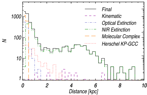
Fig. 9. Distance distribution per type: kinematic, optical extinction, near-infrared extinction, molecular complex association, and Herschel HKP-GCC.
