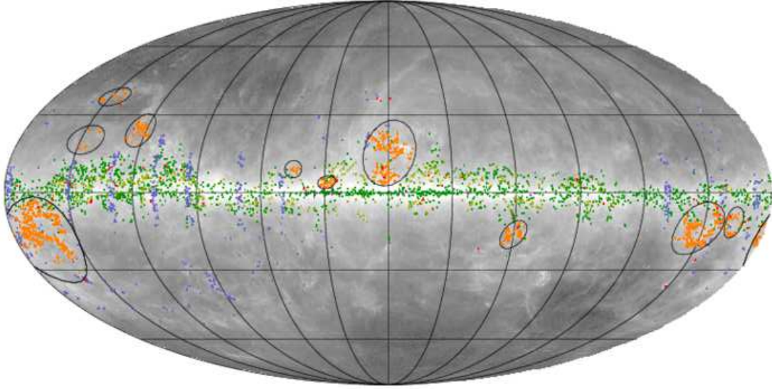
Fig. 8. All-sky distribution of the 4655 PGCC sources for which a distance estimate with a DIST_QUALITY flag equal to 1 or 2 is available. The various types of distance estimates are defined as follows : kinematic (purple), optical extinction (blue), near-infrared extinction (green), molecular complex association (orange), and Herschel HKP-GCC (red). We also show the distribution of the 664 sources with an upper-limit estimate (DIST_QUALITY=4) provided by the near-infrared extinction method in light green. The regions covered by the molecular complexes are shown as black contours (see Table 3).
