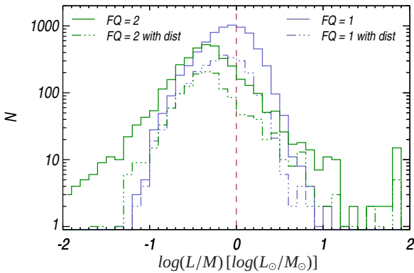
Fig. 12. Distribution of the luminosity to mass ratio of the PGCC clumps for sources with FQ=1 (blue line) and FQ=2 (green line). The dot-dot-dot-dashed line denotes the distribution for the sub-sample of sources with a reliable distance estimate.
