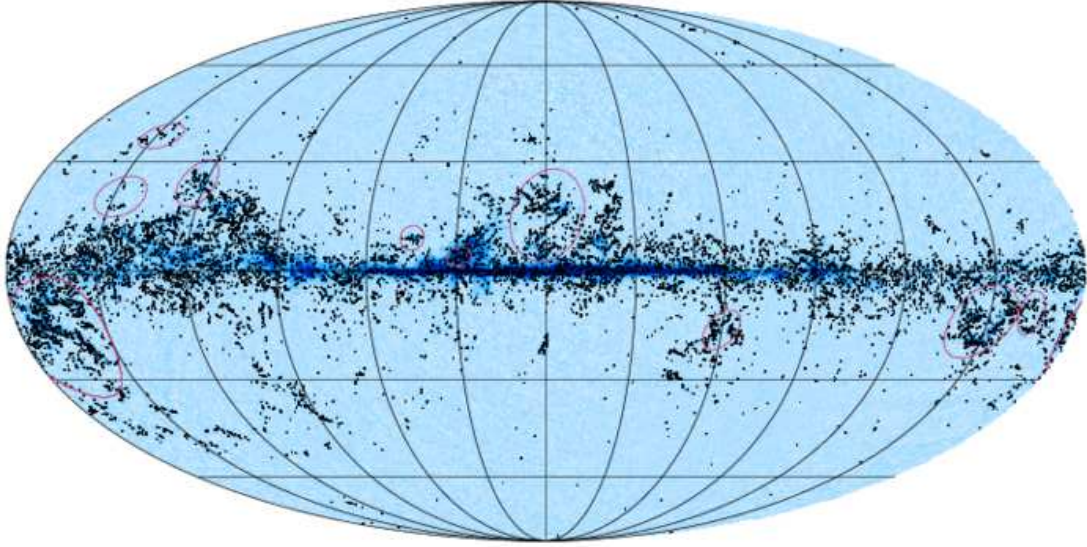
Fig. B.1. All-sky distribution of the PGCC sources with FQ=1 or 2, displayed over the Planck ^{12}\text{CO } J=1\rightarrow 0 map ranging from -5 to 30 K.kms ^{-1} . The locations of the molecular complexes used in the distance estimate procedure are shown as red circles.
