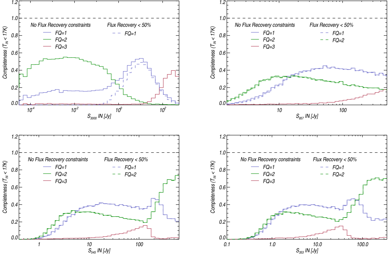
Fig. 4. Completeness (computed on a restricted sample of sources with injected temperature below 17 K) as a function of the injected flux density in the IRAS 3 THz (top left panel) and Planck upper frequency bands, 857 GHz (top right panel), 545 GHz (bottom left panel), and 353 GHz (bottom right panel). It is shown per-category of flux density quality, i.e., FQ=1, 2 and 3 categories (blue, green and pink, respectively). The completeness is also computed on a more restricted sample of sources with injected temperature below 17 K and with a flux density accuracy better than 50% (dashed lines).
