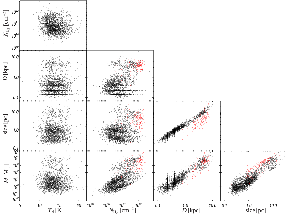
Fig. 13. Correlation plots for: temperature, column density, distance, size and mass. The black dots represent 3867 PGCC sources with a robust distance and flux density estimate. The red dots denote the IRDCs from Simon et al. (2006b) . between the following physical properties of the 3867 PGCC sources for which a robust distance estimate is available combined with a reliable flux density: temperature, column density, distance, size and mass. It is compared to the physical properties of IRDCs from Simon et al. (2006b) in red.
