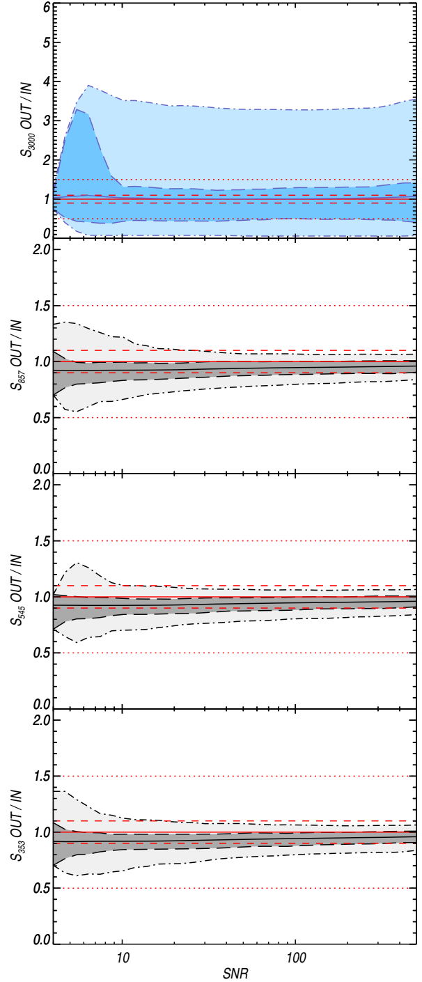
Fig. 7. Ratio of the recovered (OUT) to injected (IN) flux densities for the simulated sources detected with FQ=1 and 2. The ratio is given as a function of the detection S/N estimated from the cold residual maps. The light and dark grey shaded regions (denoted by the dot-dashed and long-dashed lines, respectively) highlight the behaviour of 95% and 68% of the sources, respectively, in each S/N bin. Note that at 3 THz ( top panel ) we only consider sources with FQ=1 , and the corresponding contours and shaded regions are highlighted in colour. The median of the ratio distributions are shown with a solid line . The 0%, 10% and 50% uncertainty levels are overlaid using a red solid, dashed and dotted line , respectively.
