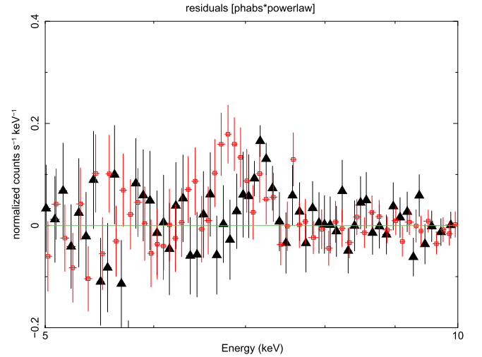
Figure 5. Residuals in units of count s -1 keV -1 of the A 2 (black triangles) and JKL (red squares) states, in the XMM-Newton first and second observations, respectively. The used model is an absorbed power law (see the text for details).
