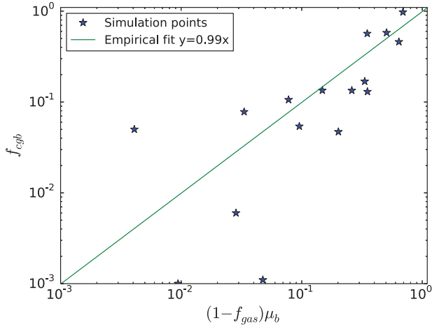
Figure 6. The fraction of central gas disc mass given to the central bulge. The blue points are simulation results and the green line is the empirical fit to the points.
