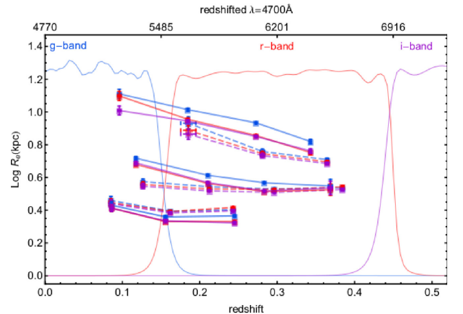
Figure D1. Size–redshift relation for the spheroids (solid lines) in the mass bins \log M_*/M_\odot = 10.4, 10.8, 11.2 and disc dominated galaxies in the mass bins \log M_*/M_\odot = 10.0, 10.4, 10.8 (dashed lines) in g (blue), r (red), and i (purple) bands.
