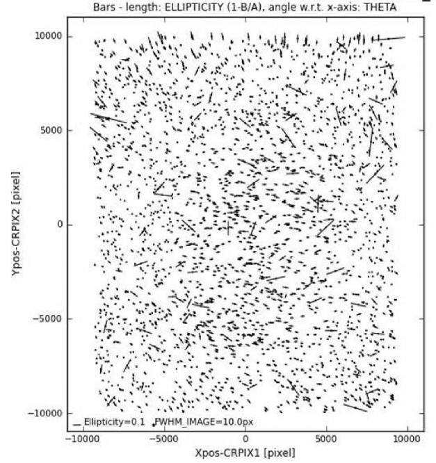
Figure 4. PSF anisotropy within the coadd KiDS_129.0-0.5 in r band. The elongation is aligned in a specific direction on the borders but random in the middle of the image.
