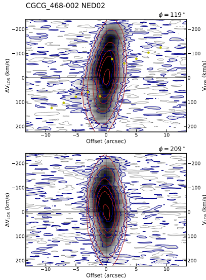
Fig. 11. Position velocity diagrams of NED02 showing the comparison between the data (blue contours, plotted at 3, 6, 9, 15, 20, 30, 40, and 50 \sigma ) and the BBarolo best-fit rotating disk model (red contours). The upper panel shows the PV diagram extracted along the major axis, and the lower panel shows the one extracted along the minor axis of rotation.
