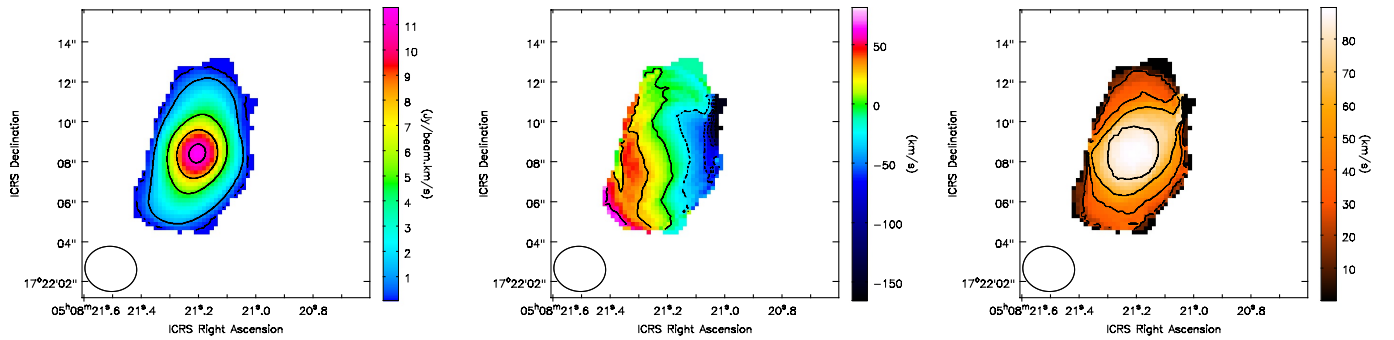
Fig. 5. Moment maps of NED02 computed from the non-PB-corrected datacube within a box of size 14'' centred at \text{RA(ICRS)} = 05:08:21.108 ; \text{Dec(ICRS)} = 17:22:08.489 , including pixels above a CO(1–0) intensity threshold of 0.009 \text{ Jy beam}^{-1} and within v \in [-500, 500] \text{ km s}^{-1} . Left: Intensity (moment 0) map, with contours plotted at [0.1, 1, 5, 8, 11] \text{ Jy beam}^{-1} \text{ km s}^{-1} . Centre: Velocity (moment 1) map, with contours plotted every 30 \text{ km s}^{-1} . Right: Velocity dispersion (moment 2) map, with contours plotted at intervals of 20 \text{ km s}^{-1} .
