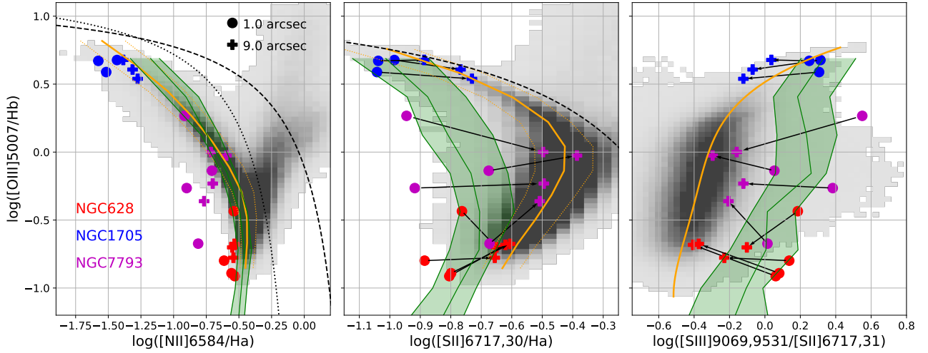
Figure 5. BPT diagrams plotting [\text{OIII}]\lambda 5007/H\beta vs. [\text{NII}]\lambda 6584/H\alpha (left), [\text{SII}]\lambda 6717,31/H\alpha (center), and [\text{SIII}]\lambda 9069,9531/[\text{SII}]\lambda 6717,31 (right). Circles show line ratios extracted from 1'' \times 1'' apertures, crosses from 9'' \times 9'' aperture. Arrows link the points relative to the same region. The grey-scale image in the left and central panels show the distribution of SDSS-DR7 galaxies, with the orange lines showing the medians of the distribution. The distribution from MaNGA galaxies (not shown) is perfectly coincident with that from SDSS. In the right panel, the grey-scale image and the orange line are from MaNGA spaxels. The dotted and dashed black lines separate galaxies dominated by star formation and by AGNs, and are from Kauffmann et al. (2003) and Kewley et al. (2001) , respectively. The green band shows the position of the H II regions in the CHAOS project from Berg et al. (2015) , Croxall et al. (2015) , and Croxall et al. (2016) , with the lines showing the 25th, 50th, and 75th percentiles.
