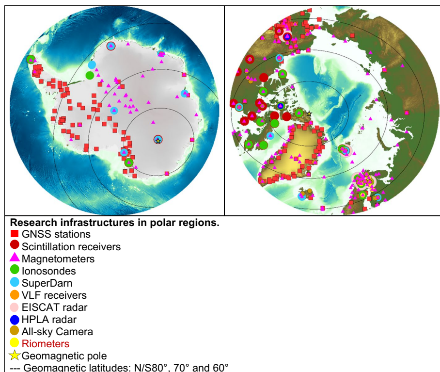
Fig. 1 Scientific instrumentation infrastructure in Antarctica and Arctic regions (selected established stations to indicate the coverage of measurements)
