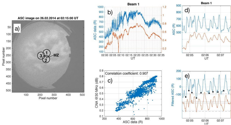
Fig. 16 Correlations between CNA and optical data are seen by Grandin et al. (2017b). Panel a Position of the KAIRA beams number 1, 2, and 3 on an example Kilpisjärvi all-sky image. Panel b Time series of the 427.8 nm auroral emission (blue) and cosmic noise absorption (orange) between 02:00 and 02:35 UT within KAIRA beam number 1. Panel c correlation between cosmic noise absorption and 427.8 nm auroral emission. Panel d as panel b, but zoomed in. Panel e high-pass-filtered optical (blue) and CNA (orange) data
