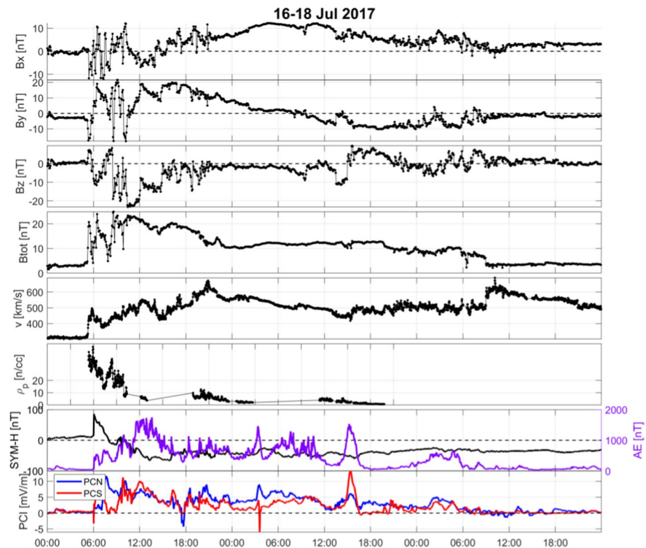
Fig. 31 Summary of the geospace characteristics during the event of 16–18 July 2017. From the top to the bottom they are plotted, vs UT: The Interplanetary Magnetic Field components ( B_x , B_y , B_z , from top to bottom) and B_{tot} , the solar wind speed ( v ) and proton density ( \rho_p ), the geomagnetic indices SYM-H, AE and PCI, the last two mostly related to auroral and polar cap conditions. PCN and PCS refer to the Polar Cap Index (PCI) at Northern (N) and Southern (S) hemispheres, respectively
