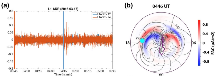
Fig. 29 a Phase variations (in radians) highlighting a scintillation observed by a receiver at Poker Flat during the storm sudden commencement; b FAC distributions from the BATSRUS MHD model (Zou et al. 2017b)
