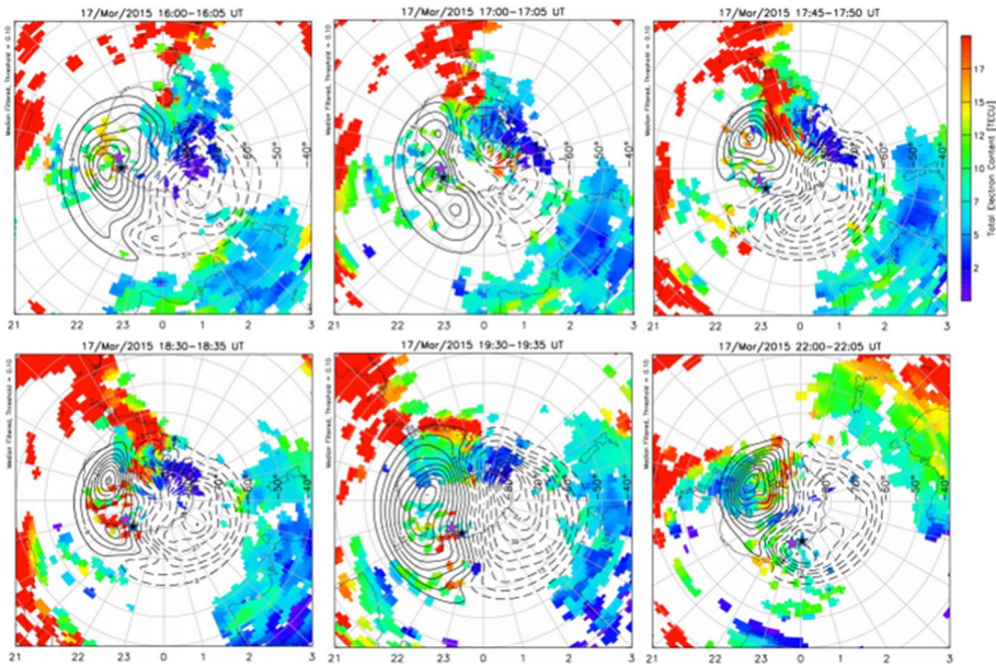
Fig. 28 Panels a–f (from top-left to bottom-right) show the TEC in the southern hemisphere at selected times (1600 UT, 1700 UT, 1745 UT, 1830 UT, 1930 UT and 2200 UT) on 17 March 2015. The SuperDARN convection pattern is overlaid on the TEC maps to facilitate comparison of the changes in the TEC along the path of convection. The location of Bharati and Davis stations are marked on the maps using pink and black stars, respectively (from Shreedevi et al. 2020)
