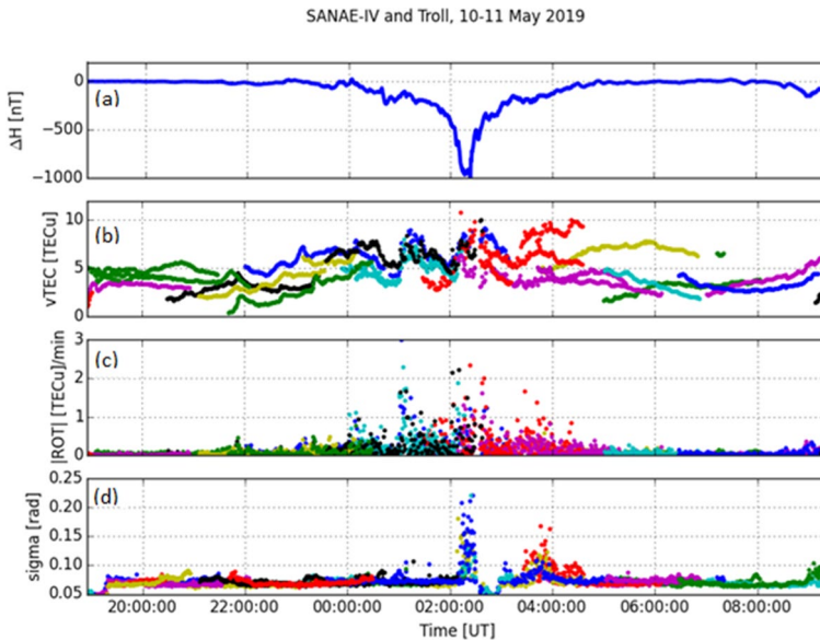
Fig. 40 a Magnetic field variations observed over SANA-IV, and b vertical TEC, c ROT and d \sigma_\phi scintillation index observed over Troll on 10–11 May 2019
