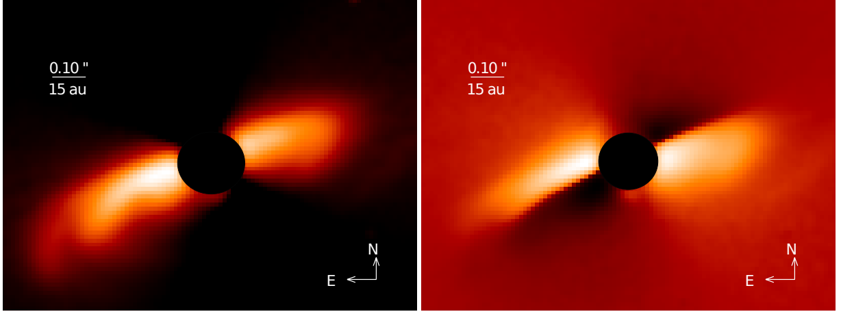
Fig. 2. IRDIS DPI Q_\varphi (left) and U_\varphi (right) images showing the close environment of RY Lup. The dark central region corresponds to the area masked by the coronagraph. The intensity scale follows the inverse hyperbolic sine.
