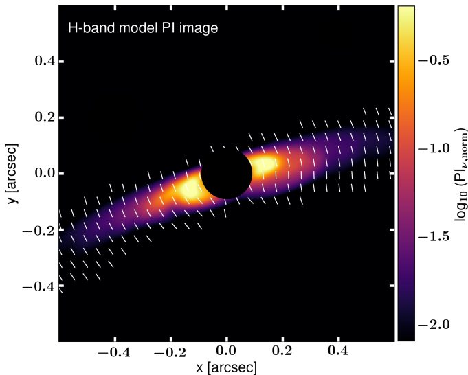
Fig. 10. Convolved polarized intensity H -band image considering a planet-induced spiral model with M_{\text{pl}}/M_{\star} = 1.4 \cdot 10^{-3} . The image is produced at an inclination of 75 deg, and a PAs of 107 deg. The inner 0.18'' are masked (black circular area) to mimic the coronagraph region. The white stripes represent the angle of linear polarization (fixed length, not scaled with the degree of polarization).
