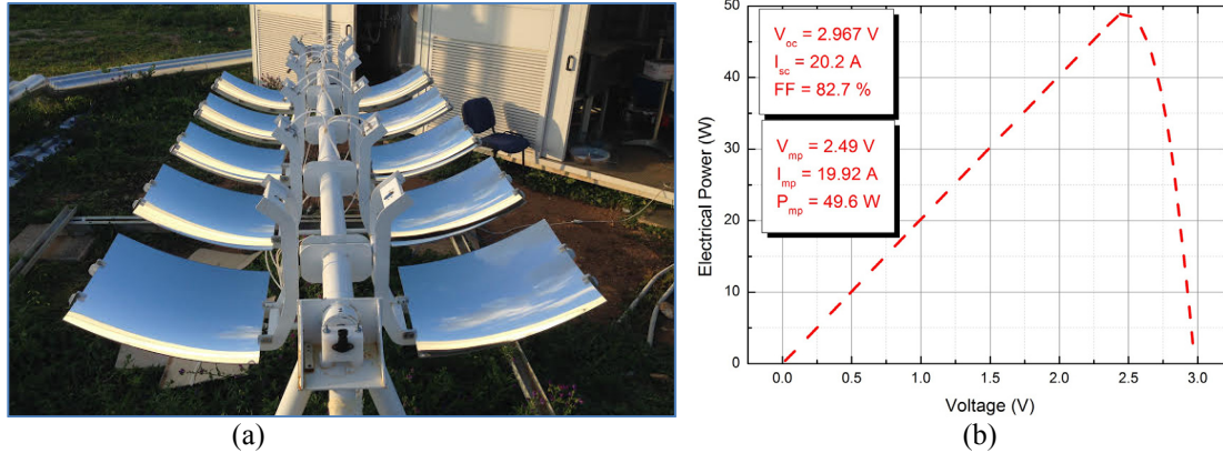
FIGURE 8. HCPV-FAE 1kWe prototype installed in the open air solar laboratory at Consorzio ARCA in the campus of the University of Palermo (a) and the characteristic curve (b) of one cell in real operation conditions @DNI=900W/m 2 .
