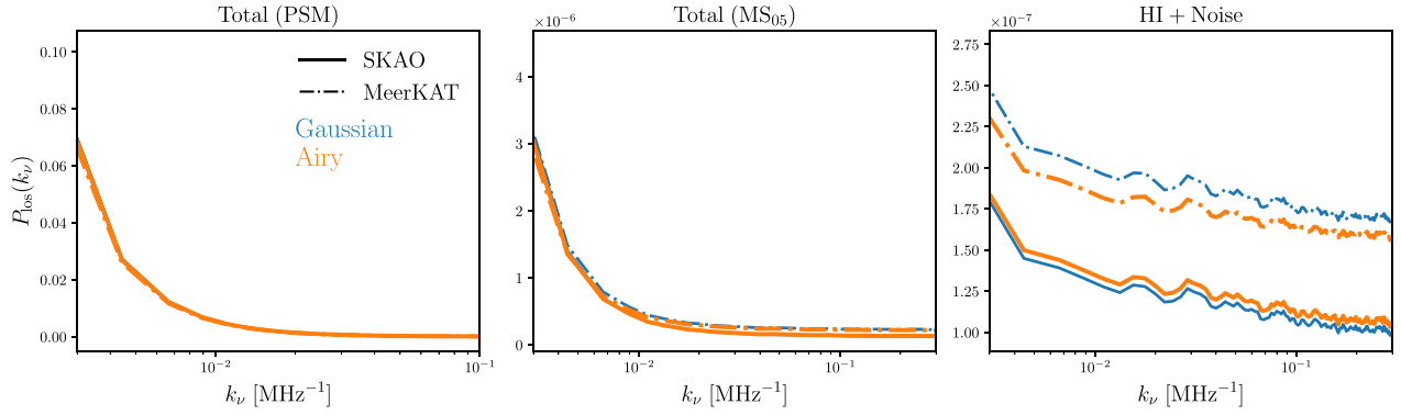
Figure 8. The line-of-sight power spectrum P_{\text{los}} for the total sky emission considering the PSM foregrounds (left) or the MS05 model (centre), compared with the H I signal plus the noise (right), for both an SKAO-MID-like survey (solid lines) and a MeerKAT-like survey (dot-dashed lines). We show results after convolution with a Gaussian beam model (in blue) and the Airy beam model (in orange).
