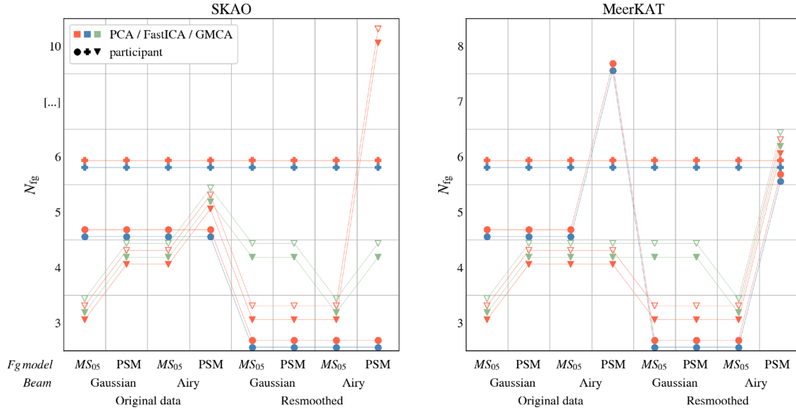
Figure 9. Graphical representation of N_{fg} used for the various cleaning methods as reported in Table A1, shown separately for the case of SKAO (left-hand panel) and MeerKAT (right). Each row represents the integer number N_{fg} used in each method, with the lines offset to facilitate reading. Each column refers to a specific data set as described by the legend below the x-axis. Different colours correspond to different cleaning methods and different symbols to the different participants who performed the cleaning (i.e. different pipelines too). In the case of mixGMCA, two values of N_{fg} need to be set: for a PCA run at the large scale and a GMCA run at small scales; we decompose the mixGMCA information into two PCA/GMCA cases that we highlight using empty symbols.
