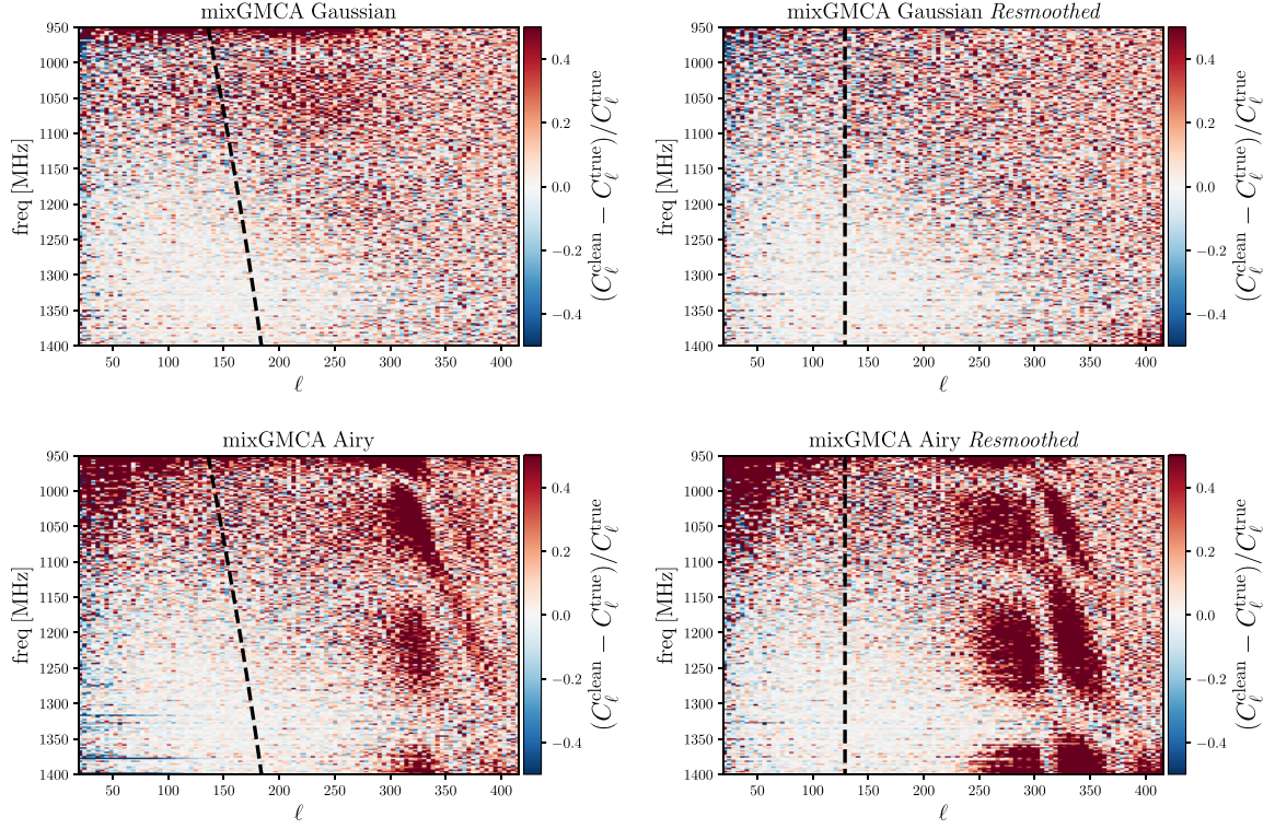
Figure 17. The estimator (C_\ell^{\text{clean}} - C_\ell^{\text{true}})/C_\ell^{\text{true}} for one of the cleaning methods (mixGMCA in this example) in the PSM and SKAO scenarios, where C_\ell^{\text{clean}} is the angular power spectrum of the cleaned maps, while C_\ell^{\text{true}} is the angular power spectrum for the input signal and noise, as a function of frequency. From top to bottom, the beam model changes from Gaussian to Airy, while from left to right is shown the effect of resmoothing. For reference, the black dashed line in all panels indicates the angular scale of the FWHM of the telescope beam. After resmoothing, this scale is constant with frequency.
