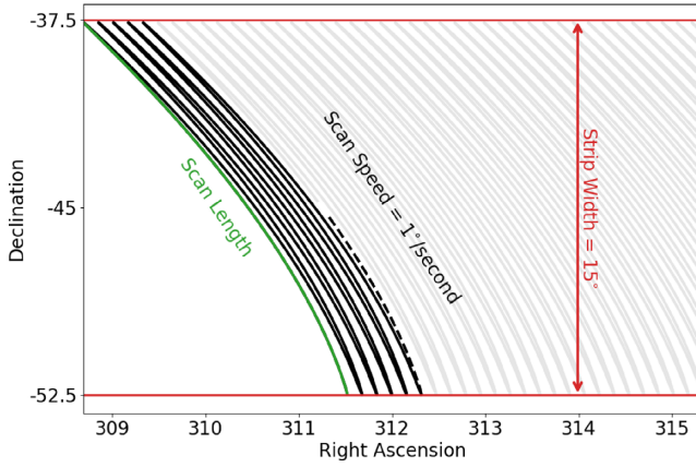
Figure 4. Example of the constant elevation scanning strategy used to map out the strip centred on -45^\circ declination. For visualization purposes, we highlight the first scan in this example in green , which defines a single scan length, the black lines represent the area already scanned, while the faint black lines represent the upcoming scans. The red lines mark the declination boundaries of the strip, which has a width of 15^\circ . Each strip has the same width and scanning speed.
