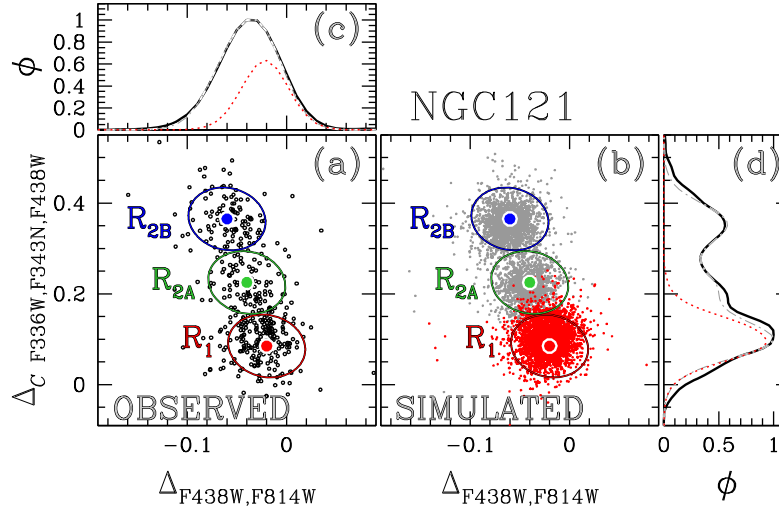
Figure 4. Procedure to estimate the fraction of 1G, 2G A , and 2G B stars in NGC 121. The observed ChM is reproduced in panel (a), while panel (b) shows the simulated ChM where simulated 1G stars are coloured in red. The three elliptical regions, namely R 1 , R 2A , and R 2B that we used to estimate the population ratios, are superimposed on both ChMs and are coloured in red, green, and blue, respectively. The continuous black lines and the grey dashed-dotted lines plotted in panels (c) and (d) show the \Delta_{F438W,F814W} and \Delta_{CF336W,F343N,F438W} kernel-density distributions of stars in the observed and simulated ChM, respectively. The red-dotted lines are the kernel-density distributions of simulated 1G stars.
