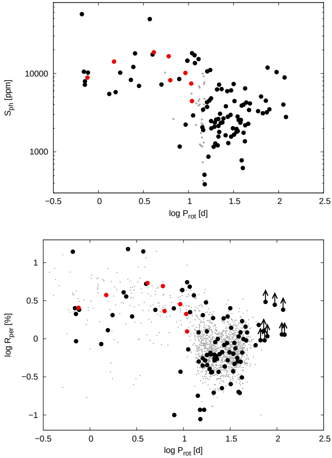
Fig. 16. Photometric activity diagnostics versus rotation period for M stars. Red dots – M stars in our sample; black dots – K2 M dwarf sample of Stelzer et al. (2016); gray dots – field M dwarfs in the sample by Mathur et al. (2014a) in the top panel and field M dwarfs from McQuillan et al. (2013) in the bottom panel .
