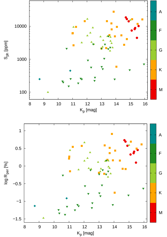
Fig. 17. Photometric activity diagnostics versus Kepler magnitude for the stars in our Kepler/XMM-Newton sample divided in spectral type bins. Top: S_{\text{ph}} versus Kepler magnitude; Bottom: \log R_{\text{per}} versus Kepler magnitude.
