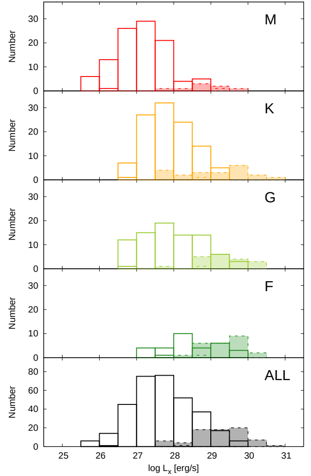
Fig. 7. Distribution of the X-ray luminosity in the energy band 0.2 – 2.0 keV, for the 102 main-sequence stars of the Kepler - XMM-Newton sample (hatched histograms) and for the NEXXUS stars from Schmitt & Liefke (2004) (solid line) for each spectral type class separately and for all spectral types combined.
