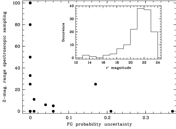
Fig. 17. Percentage of spectroscopic redshifts within r_{500,\text{scal}} that are found in the two-magnitude interval fainter than the BCG, as a function of the uncertainty on the probability for a cluster to be a fossil group (given in Table 11). Inset: r' band magnitude histogram of the galaxies without a spectroscopic redshift, and within the two-magnitude range of our FG candidates.
