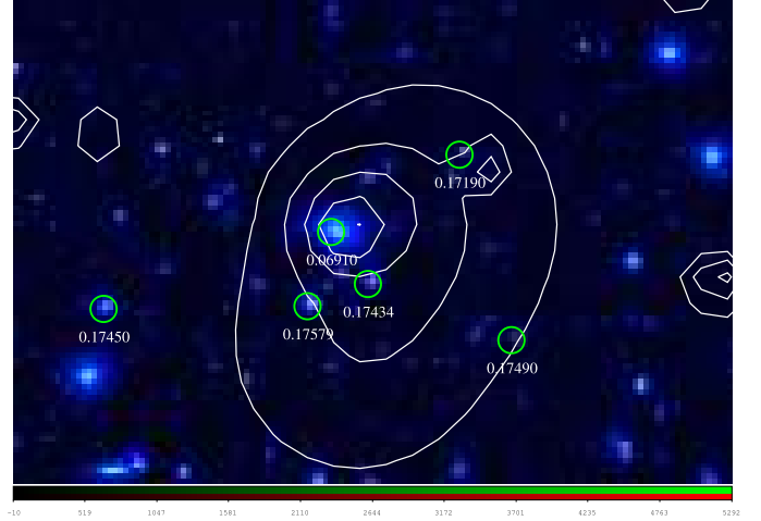
Fig. B.1. CFHTLS i' band 4.5' \times 3' image around the XLSSC 035 confirmed z = 0.174 cluster. Green circles represent the member galaxies plus the bright foreground galaxy discussed in the text. White contours are for the X-ray emission.
