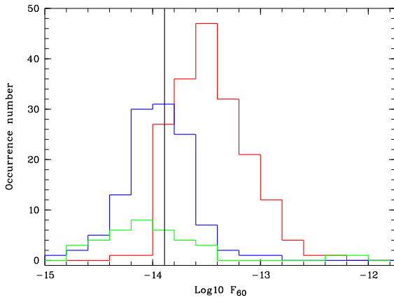
Fig. 9. X-ray flux ( F_{60} in log unit of \text{erg s}^{-1} \text{cm}^{-2} , within a 60'' radius in the [0.5\text{--}2] keV band) distribution for the clusters having a spectroscopic redshift. Red histogram: the C1 sample; blue histogram: the C2 sample; green histogram: the C3 sample. The black vertical line is the estimated reference flux completeness limit of 1.3 \times 10^{-14} \text{ erg s}^{-1} \text{cm}^{-2} .
