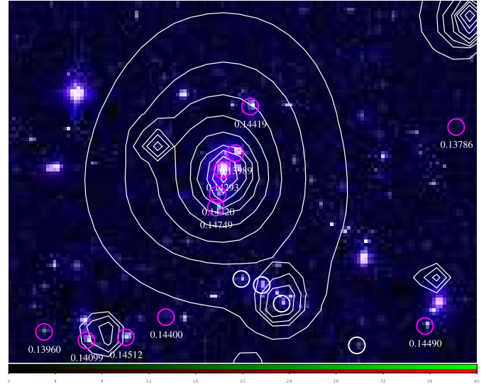
Fig. B.2. CFHTLS i' band 5.5' \times 3.5' image around the XLSSC 041 confirmed z = 0.142 cluster. Magenta circles represent the member galaxies. White circles are the galaxy members of the background cluster at z = 0.557 . White contours are for the X-ray emission.
