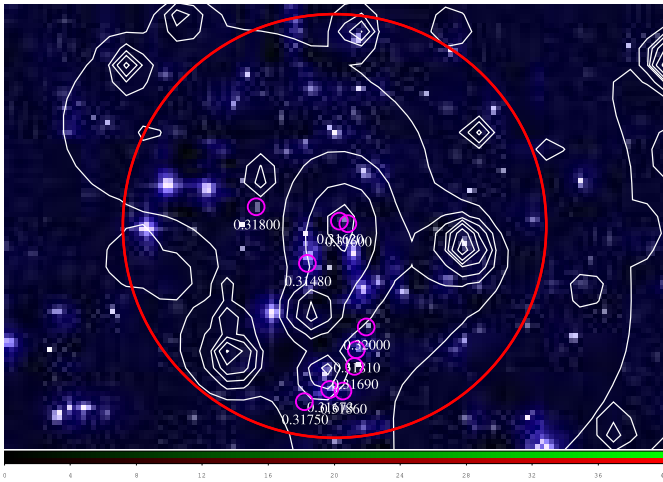
Fig. B.7. CFHTLS i' band 6.5' \times 4.5' images of two superposed structures. Magenta circles represent the member galaxies of the two structures at z = 0.263 (upper panel) and at z = 0.317 (bottom panel). The large red circle represents a 500 kpc radius area. White contours are for the X-ray emission.
