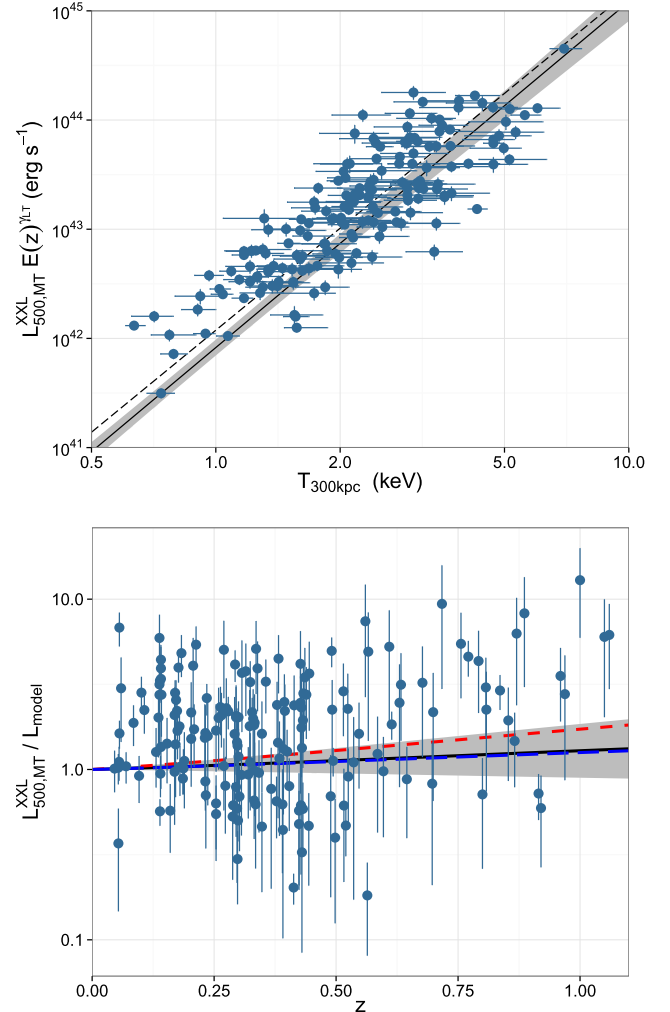
Fig. 10. Upper panel: luminosity–temperature relation with the best-fitting models. The light blue circles show the XXL-C1-GC clusters; the best-fitting model (including selection effects) is shown by the solid black line, the 1\sigma uncertainty represented by the grey shaded region. The best-fitting model fitted to the data using the BCES regression is shown as the dashed line. Bottom panel: evolution of the luminosity–temperature relation for XXL-C1-GC. The XXL-C1-GC clusters are represented by the light blue circles and the best-fitting model is given by the black solid line; the grey shaded region highlights the 1\sigma uncertainty. The “strong” and “weak” self-similar expectations are given by the red dashed and blue dashed lines, respectively.
