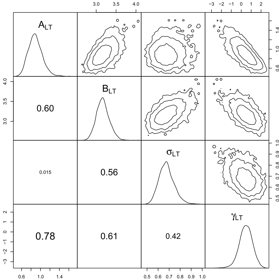
Fig. 11. Scatterplot matrix for the fit of the luminosity–temperature relation of the XXL-C1-GC sample. The posterior densities are shown along the diagonal; the 1 \sigma , 2 \sigma , and 3 \sigma confidence contours for the pairs of parameters are shown in the upper right panels . The lower left panels show the Pearson's correlation coefficient for the corresponding pair of parameters (text size is proportional to the correlation strength).
