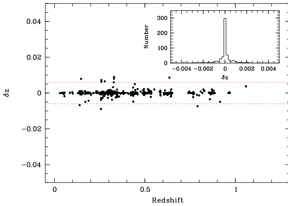
Fig. 2. Redshift difference versus redshift for the galaxies (at < \pm 3 \times \sigma_{v,200} from the cluster mean redshift and within one Virial radius) measured twice within the spectroscopic survey. The two red dotted lines represent the \pm 3 \times 600 \text{ km s}^{-1} level. We also give the histogram of the redshift difference within the [-0.005, 0.005] interval.
