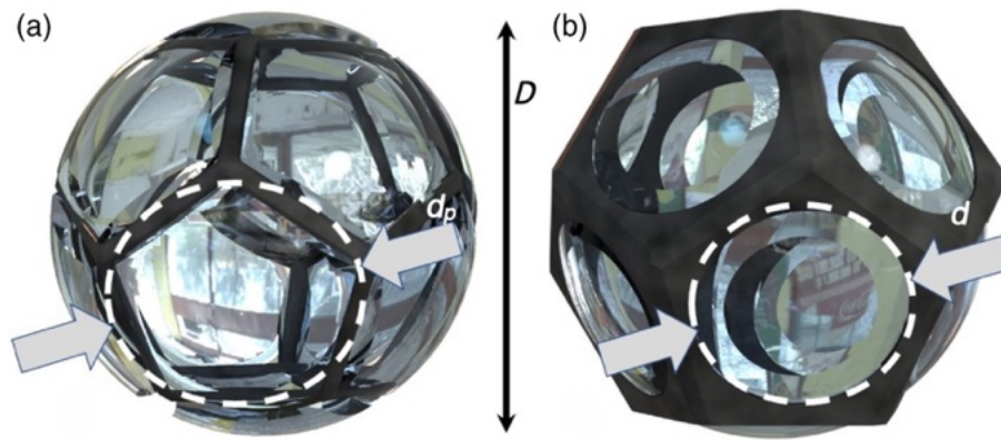
Fig. 4 Realistic representation of the telescope assembly. Because the instrument is, geometrically, a dodecahedron, the lenses could be either pentagonal or circular in shape. The pentagon outer diameter d_p and surface are 24% and 16%, respectively, greater than the circle ones: (a) pentagonal shape lenses and (b) circular shape lenses.
