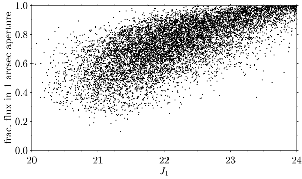
Fig. 7. Fraction of flux contained in a 1'' diameter aperture, against 1'' J -band magnitude, measured for the COSMOS sample. The flux fractions are determined by integrating de Vaucouleurs profiles.
