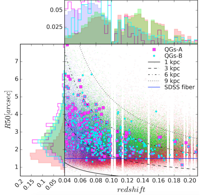
Figure A1. The size-redshift relation for our sample and quenching candidates. The horizontal blue line represents the radius of the SDSS fibre aperture, while the black curves represent the kpc/arcsec relations obtained from the adopted cosmology.
