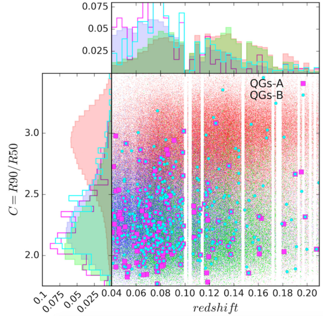
Figure 18. The light concentration–redshift relation for our sample and QGs. The layout is the same of Fig. 13.
