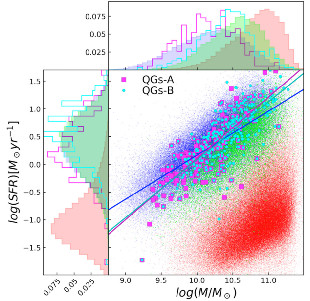
Figure 16. The \log(\text{SFR}_{\text{tot}}) as a function of the stellar mass. The layout is the same of Fig. 13. The blue straight line represents the main sequence (MS) of the SF-Alldet sample, while the magenta and cyan ones are the MS of QGs-A and QGs-B, respectively.
