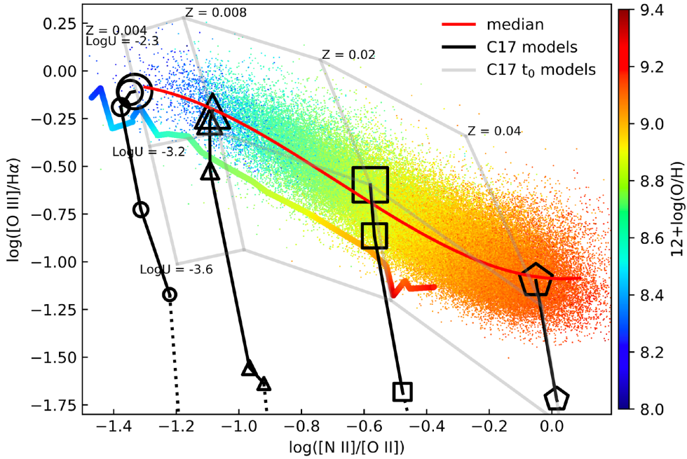
Figure 4. \log([O \text{ III}]/H\alpha) versus \log([N \text{ II}]/[O \text{ II}]) diagram. The colour of the dots shows the metallicity estimate 12+\log(O/H) by Brinchmann et al. (2004) and the colorful line represents the dispersion at 3\sigma of the \log([N \text{ II}]/[O \text{ II}]) for a given value of 12+\log(O/H) . The red curve represents the median of the relation. Superimposed in grey is reported a grid of zero-ages C17 models with different metallicities and ionization parameters, while in black are shown the evolutive tracks by C17 (circles for Z = 0.004 , triangle for Z = 0.008 , square for Z = Z_{\odot} = 0.02 , pentagon for Z = 0.04 ), where the size of the symbol is reported in time-step of 1 Myr with decreasing sizes.
