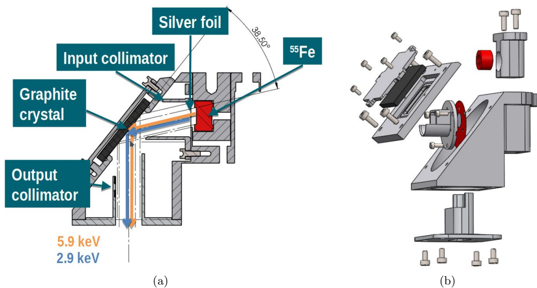
Figure 7. Cut-out (a) and exploded (b) view of Cal A.
