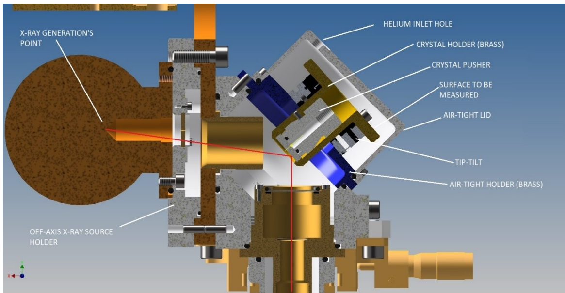
Figure 3. Cross section of the polarized calibration source.
