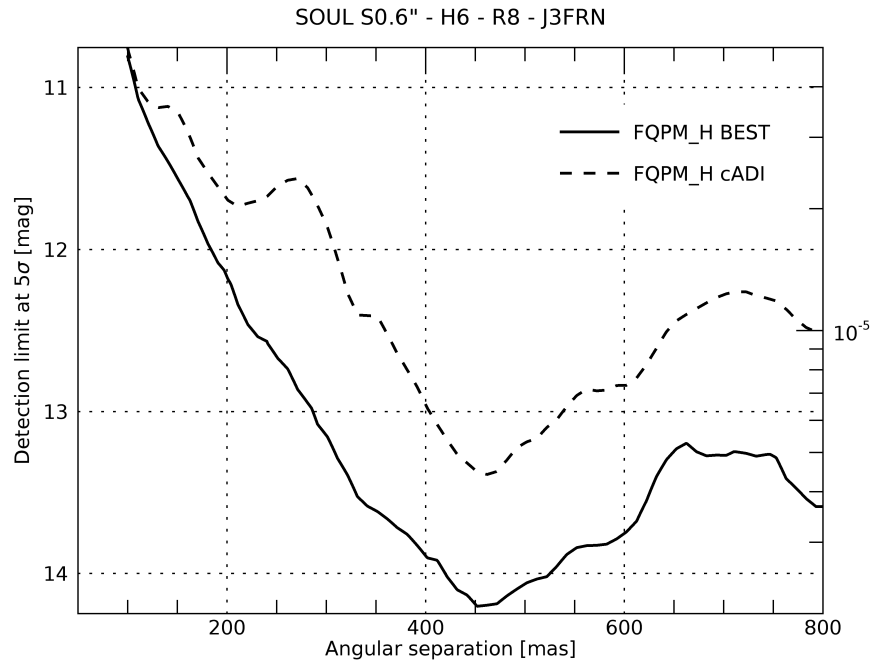
Figure 2. Detection limit in high SR regime with the FQPM obtained with classical ADI compared to the optimized data processing algorithm described in Carolo and Vassallo in prep.
