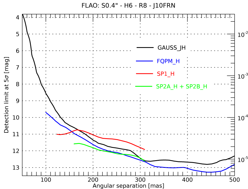
Figure 4. Detection limit in high SR regime for those coronagraphs that have been selected for implementation with FLAO system.
