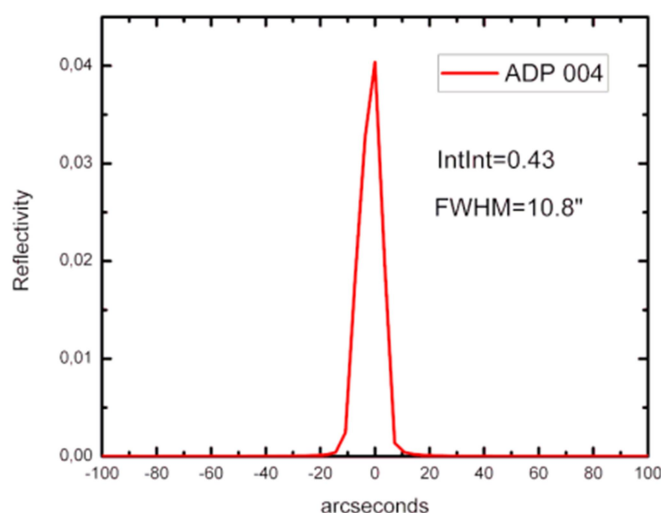
Figure 3 Experimental ADP (004) CuK \alpha diffraction profile measured at Philips MRD diffractometer with a Bartels 4xGe220 monochromator.
