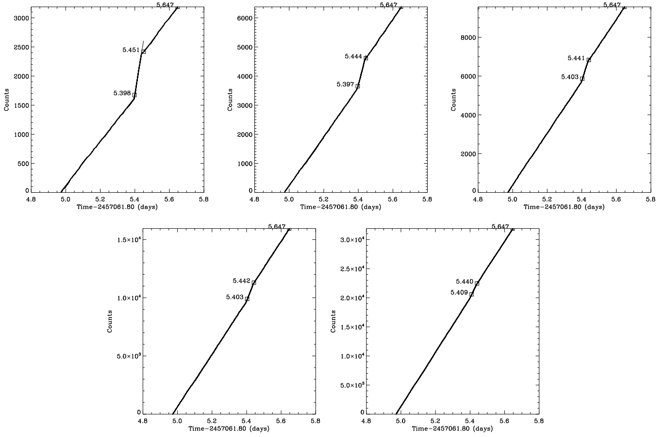
Fig. C.1. Simulated sequence of the arrival time of X-ray photons, adopting (from top-left panel to bottom-right panel) a quiescent count rate of 0.05 \text{ count s}^{-1} , 0.1 \text{ count s}^{-1} , 0.15 \text{ count s}^{-1} , 0.25 \text{ count s}^{-1} , and 0.5 \text{ count s}^{-1} .
