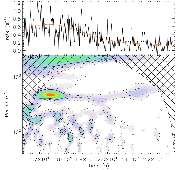
Fig. 29. Top panel: observed light curve during the flare in HCG 273 overplotted with the flare global shape obtained by fitting a third degree polynomial to the binned (10 s) light curve. Bottom panel: wavelet power spectrum obtained during the flare, with dotted, dashed, and solid contours marking peaks with 68%, 95%, and 99% confidence level, respectively. The hatched area is the “cone of influence” (see Sect. 5.2).
