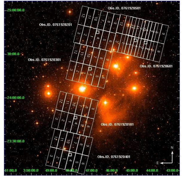
Fig. 1. DSS2-red 2^\circ \times 2^\circ image centered on the Pleiades. The detector footprints of the XMM pointings analyzed here and their associated Obs.IDs. are shown.
