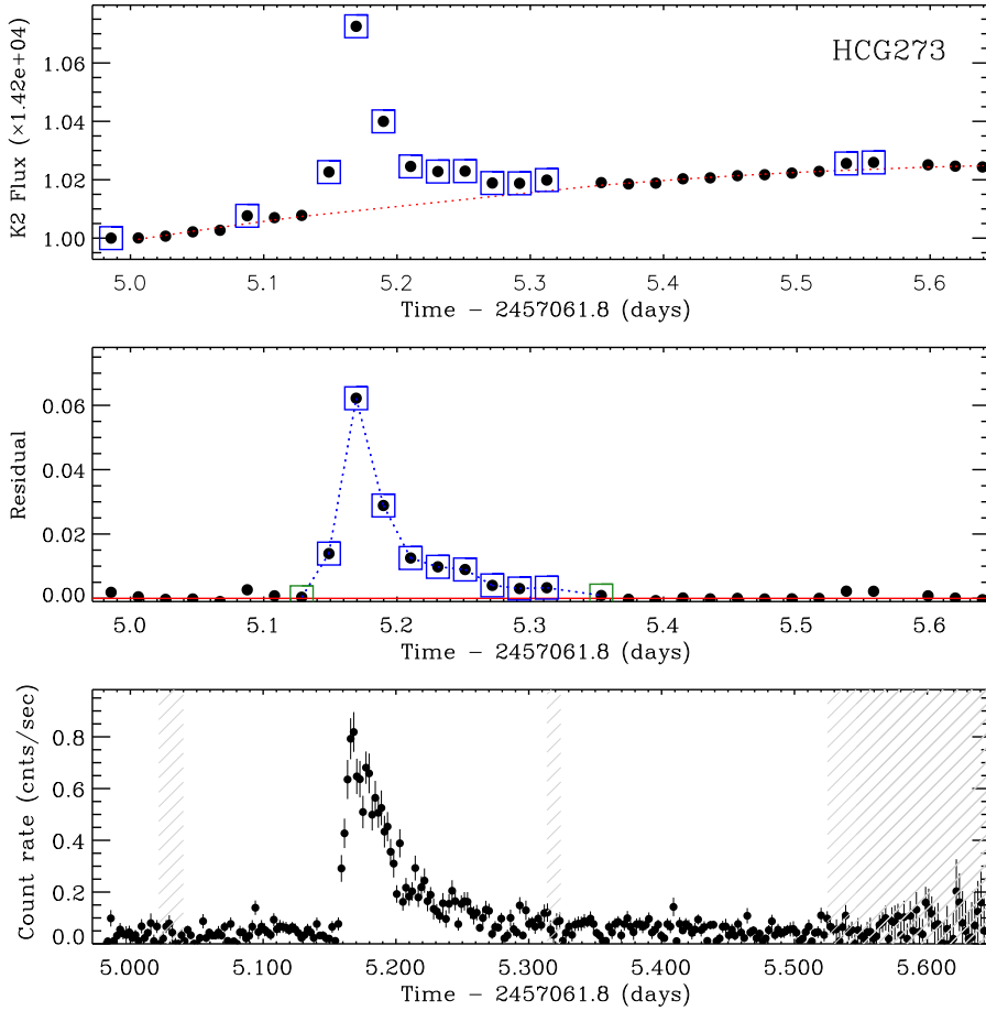
Fig. 3. Light curves of HCG 273. Top panel: K2 light curve. The error bars of K2 data points are smaller than the plot symbols. The red dotted line marks the polynomial used to fit the quiescent light curve and is limited to the portion of the K2 light curve for which the fit is performed; the blue squares mark the points corresponding to the flare. Central panel: residuals of the K2 light curve from the best-fit polynomial function limited in the portion of the light curve where the fit is performed (limited by the vertical dotted lines). The green squares mark the K2 points just before and after the flare. Bottom panel: combined background-subtracted MOS+PN X-ray light curve. Shaded regions are “bad time intervals” in at least one EPIC detector.
