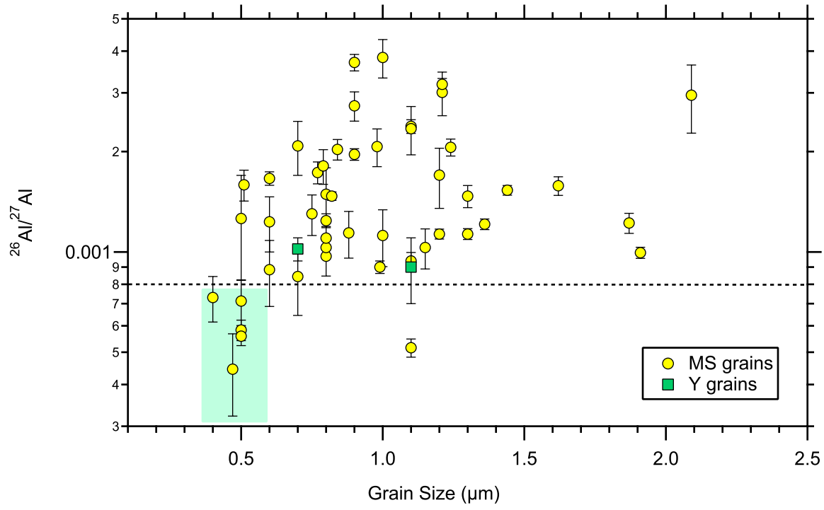
Figure A5. Plot of ^{26}\text{Al}/^{27}\text{Al} ratio versus grain size for the MS and Y grains from this study.
