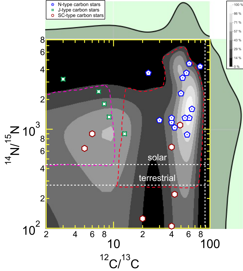
Figure A4. Observations for different types of carbon stars as shown in Fig. 3 are overlaid on the probability distribution (in grayscale colormap) of the post-Hyperion data for our 47 MS and Y grains (red dashed line region) and the pre-Hyperion data for our seven AB2 grains (fuchsia dashed line region).
