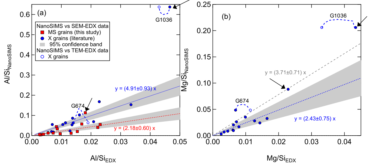
Figure A7. (a) Plot of Al/Si ratios determined by NanoSIMS versus those by SEM- and TEM-EDX for MS grains from this study and X grains from Liu et al. (2018b). A blue dashed curve connects TEM-EDX (open symbols) and SEM-EDX data (filled symbols) for the same grain. Black arrows denote grains that were excluded from the respective linear fits. (b) The same as (a) but for Mg/Si ratios. The grayscale dashed line represents the linear fit to all the grain data, and the blue dotted line is the linear fit to all but two grains (highlighted by black arrows).
