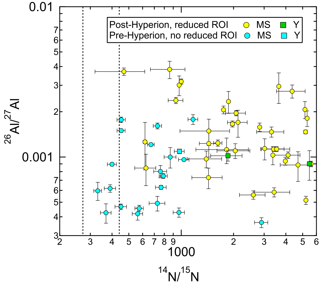
Figure A2. Plot of ^{26}\text{Al}/^{27}\text{Al} versus ^{14}\text{N}/^{15}\text{N} comparing the two sets of data for MS and Y grains from this study. Reduced ROI and no reduced ROI denote the cases of deducing initial ^{26}\text{Al}/^{27}\text{Al} by excluding adjacent Al contamination using a small ROI and by including all Al signals contained within the SiC grain, respectively.
