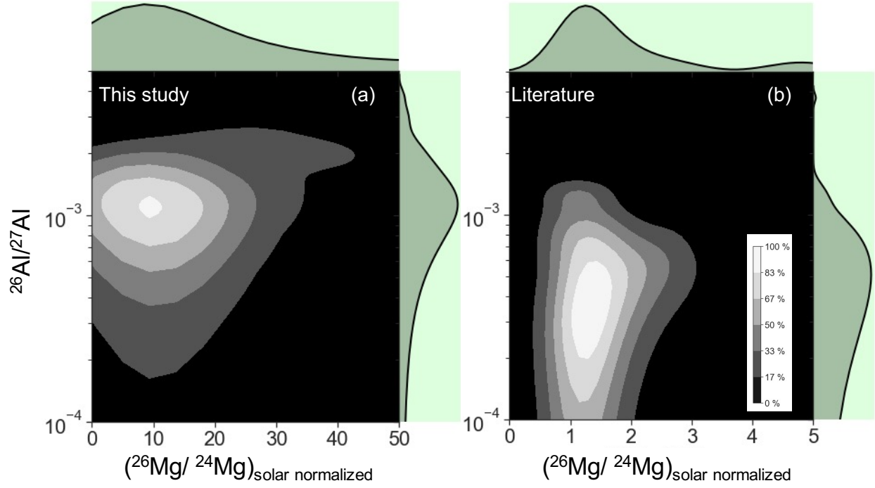
Figure A3. The probability distributions of ^{26}\text{Al}/^{27}\text{Al} versus ^{26}\text{Mg}/^{24}\text{Mg} normalized to the solar value for MS and Y SiC grain data from this study in (a) and Huss et al. (1997) in (b).
