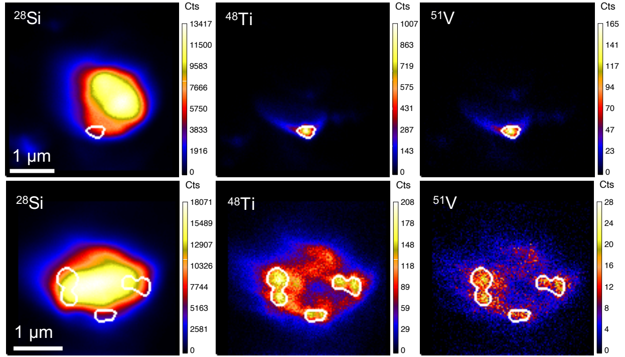
Figure A6. NanoSIMS ion images of MS grains M1-A2-277 (upper panel) and M1-A3-338 (lower panel). The white contours highlight Ti,V-hotspots within the grains.
