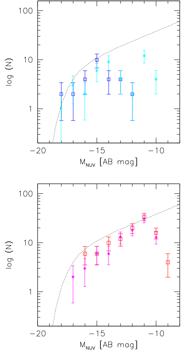
Figure 12. The NUV LFs of NGC 5846 group splitted in late-type galaxies (top), and ETGs (bottom), compared to those of the Virgo cluster (asterisks and dotted line as in Fig. 11) from Boselli & Gavazzi (2014, their fig. 14).
