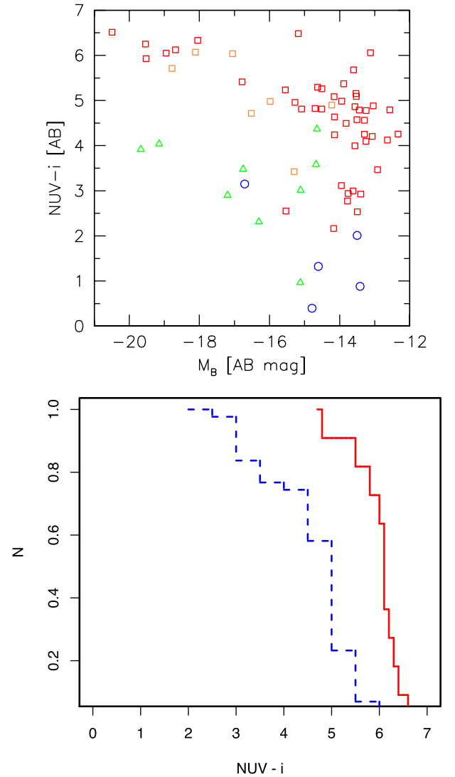
Figure 7. Top: the M_B versus NUV-i CMD of the group members. Symbols are as in Fig. 6. Bottom: cumulative distributions of NUV-i of dwarf (blue dashed line) and normal (red continuous line) ETGs in our group; according to the Kolmogorov–Smirnov test the null hypothesis, that the two distributions are drawn from a same parent distribution, can be rejected at a confidence level > 99 per cent.
