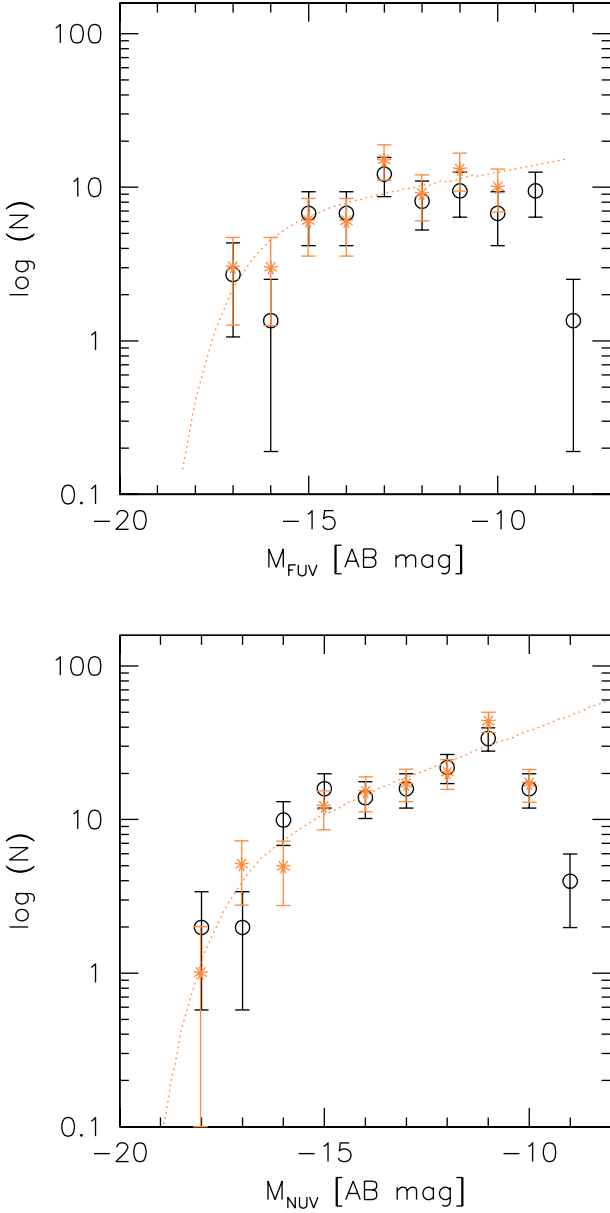
Figure 11. The FUV and NUV LFs of NGC 5846 group (open circles) compared to those of the Virgo cluster (asterisks; dotted line shows the fit limited to -13 mag by Boselli & Gavazzi (2014). LFs have been normalized to include the same galaxy number as Virgo, i.e. 135 in NUV and 65 in FUV as in Boselli & Gavazzi (2014).
