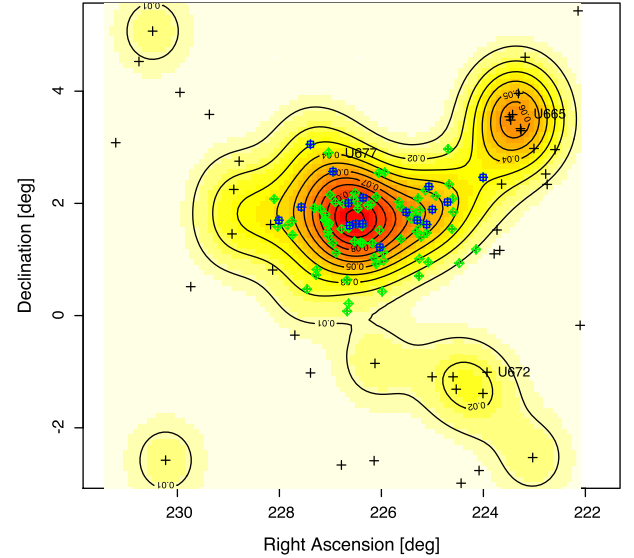
Figure 4. Spatial distribution of galaxies within a box of 4 \times 4 \text{ Mpc}^2 centred on NGC 5846 (shaded yellow/red area). Blue squares show the members of the group listed in the catalogue of Ramella et al. (2002) and green diamonds indicate the added members (Section 2). The map is normalized to the total density. The 2D binned kernel-smoothed number density contours for the galaxies with m_B \leq 15.5 \text{ mag} (circle + cross) are shown. The value of m_B = 15.5 \text{ mag} is the magnitude limit of the Ramella et al. (2002) catalogue.
