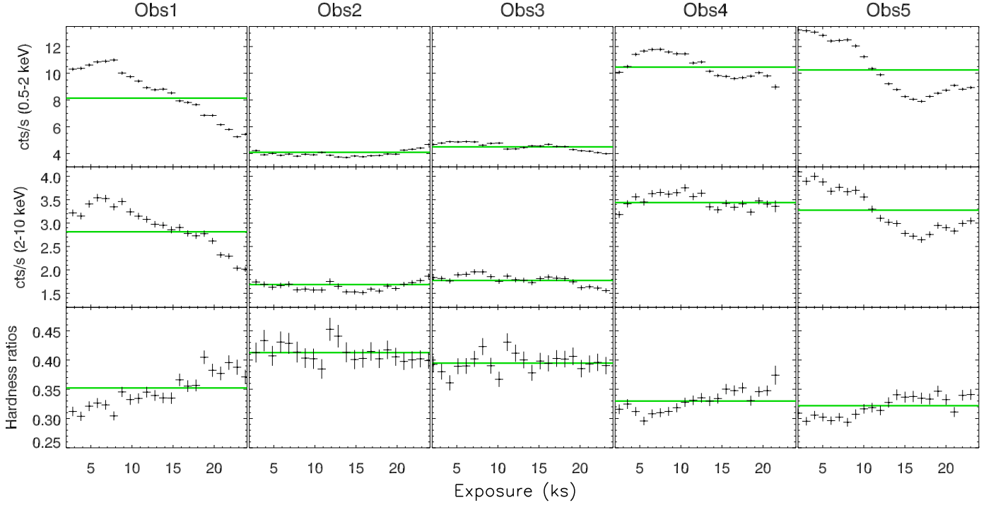
Figure 3. The XMM-Newton light curves in the 0.5-2 keV and 2-10 keV energy bands are shown in the top and middle panels respectively. Bottom panels display the ratios between the hard light curves and those computed in the soft band. The adopted time binning is 1 ks for all the observations, and the solid green lines account for the average count rates within each pointing.
