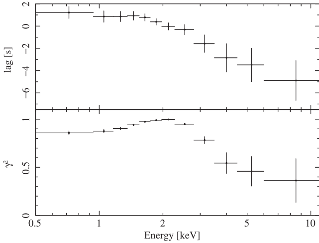
Figure 9. Upper panel: time lags at the QPO frequency (8 mHz) computed in each energy bin with respect to the reference energy band (i.e. the entire EPIC-pn energy band excluding each time the energy bin where the lag is calculated). Lower panel: the corresponding cross-correlation linear coefficient. Uncertainties are given at 68 per cent confidence level.
