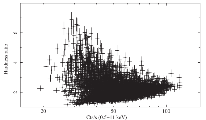
Figure 3. Hardness–intensity diagram, extracted from the light curves of Fig. 2. The source intensity is calculated in the 0.5–11 keV energy band.
