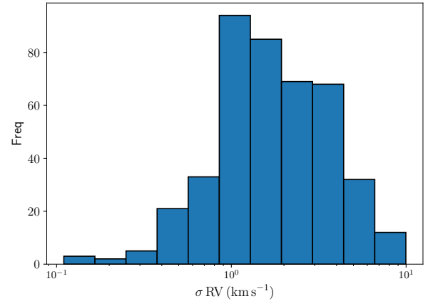
Fig. 3. Histogram of the RV standard deviation, in log scale, for the OCs with at least three members.
