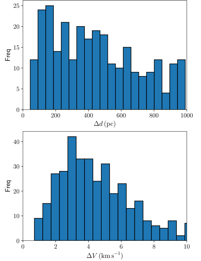
Fig. 12. Histogram of the distance between nearest neighbours in the high-quality sample ( upper panel ) and the same in velocity ( lower panel ).
