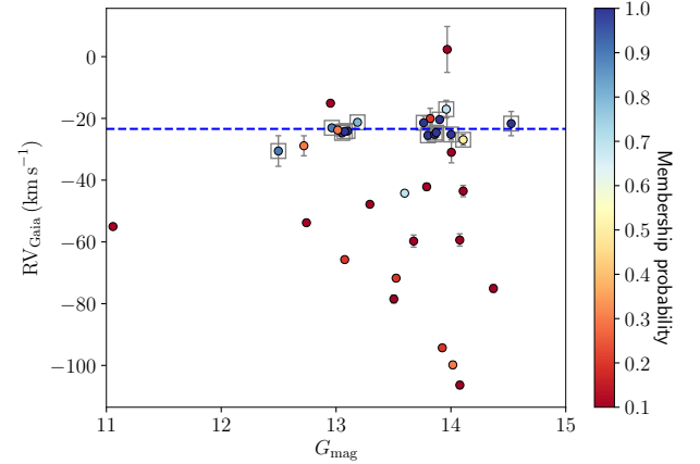
Fig. 2. Distribution of RV as a function of G magnitude for the 36 members of Skiff J0058+68.4 with a colour code corresponding to the membership probability, shown as an example. The error bars are the RV uncertainties provided in the Gaia DR2 catalogue. The 15 stars used for the calculation of the weighted RV mean are shown as open squares. The mean value, -23.4 \text{ km s}^{-1} , is shown as a blue dotted line.
