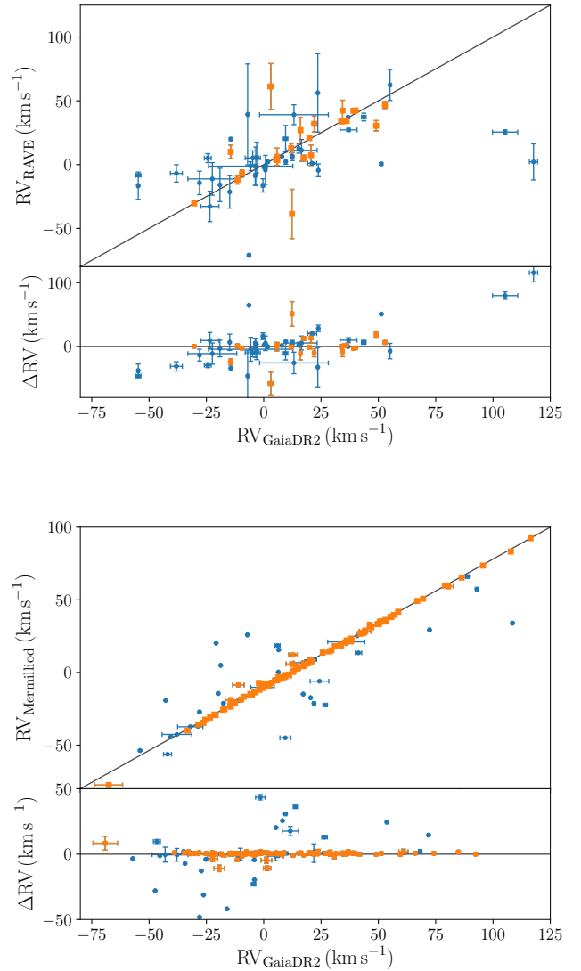
Fig. 5. Comparison of mean RV from Gaia DR2 with those from Conrad et al. (2014) using RAVE data ( upper panel ) and from ( Mermilliod et al. 2008, 2009; lower panel ). The OCs with at least three members in each catalogue are shown in orange. The error bars combine the uncertainties of both catalogues.
