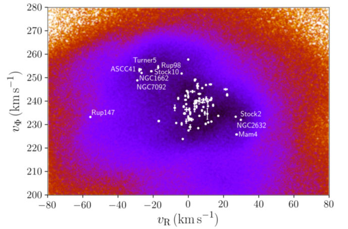
Fig. 8. Velocity distribution of nearby OCs (dist \leq 500 pc) in (V_R, V_\phi) , superimposed on field stars in the same volume around the Sun taken from Gaia Collaboration (2018c). The most extreme OCs are indicated, in particular, the two groups listed in Table 2.
