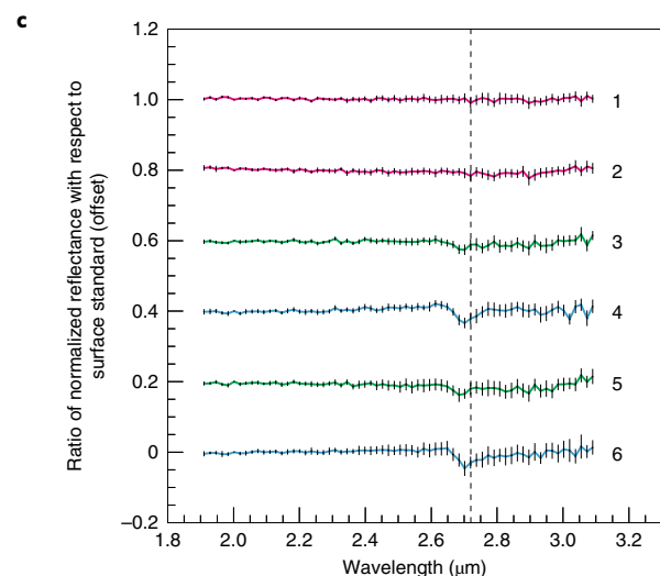
Fig. 1 | NIRS3 observations of the SCI crater region. a , Context image taken by the ONC-T camera. The dashed semi-circle represents the rim of the SCI crater 4 . The arrows indicate the motion of NIRS3 footprints during three descent operations. b , NIRS3 spectra averaged over regions corresponding to the coloured boxes shown in a . The colour of each site represents its surface characteristics: magenta, green and cyan are the ejecta-free region, ejecta-rich region outside the crater and ejecta-rich region inside the crater, respectively. Error bars are 1σ within the boxes. Individual spectra of each site are shown in Extended Data Fig. 1. c , Ratios of the normalized spectra shown in b to the ones of the surface standard observed on the day before. The spectra are normalized and vertically shifted for clarity. The dashed vertical lines at 2.72 μm denote the peak wavelength of the OH absorption of the spectra in b .
