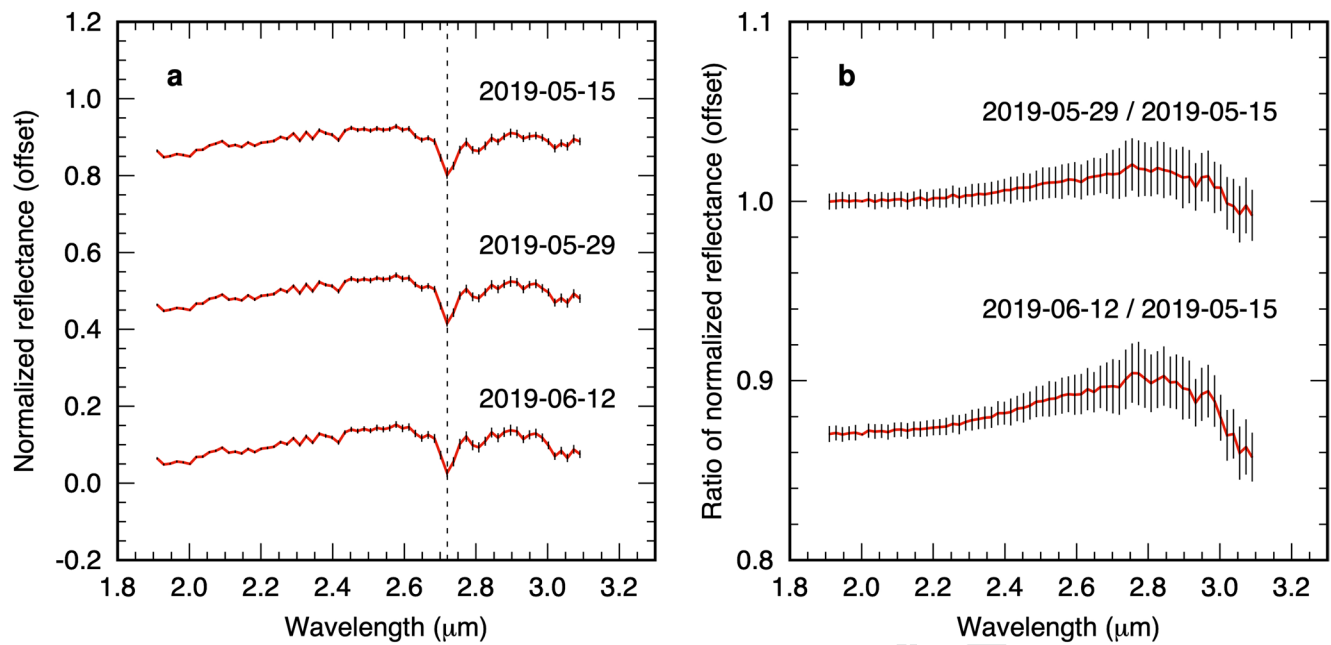
Extended Data Fig. 4 | NIR53 spectra of the surface standard. a , Spectra averaged over regions having the similar surface temperature to the SCI crater region. The details of these spectra are listed in Extended Data Fig. 3. b , Ratios between the normalized spectra shown in a . The non-flat shape of the ratio-spectra indicates the residual of thermal correction. The spectra are normalized and vertically shifted for clarity. Note that the vertical scale of b is much larger than that of a to show the curvature and uncertainties of the ratio-spectra.
