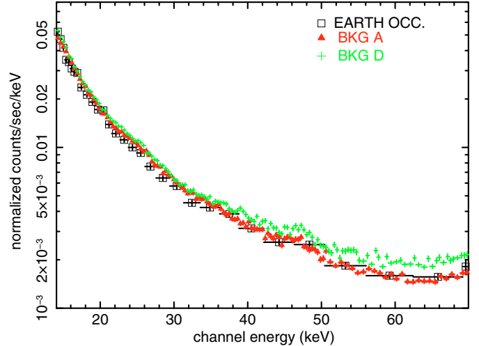
Fig. 2. Comparison between the quick (bkgA, red triangles) and the tuned (bkgD, green crosses) backgrounds with the Earth occultation spectra (black squares). The BkgD spectrum is above both the bkgA and the Earth data. The tuned background clearly overpredicts the real NXB, in particular above 35 keV.
