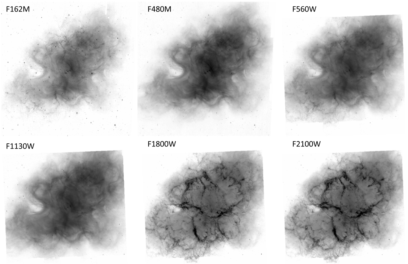
Figure 2. The NIRCam and MIRI imaging mosaics of the Crab Nebula with the dominant emission components listed in Table 1. The size of each mosaic is 4'.9 \times 5'.5 , and they are oriented with north up.
