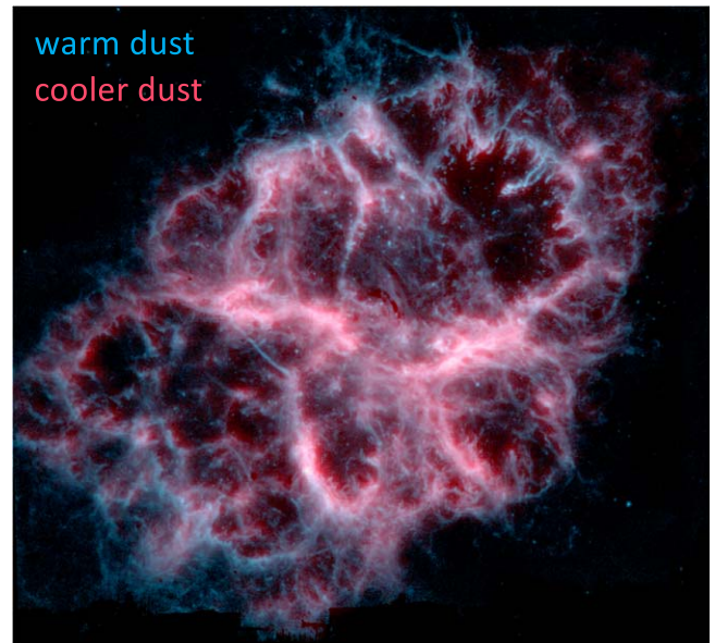
Figure 12. A color-composite image with the warm dust component from JWST shown in blue and the Herschel 70 \mu\text{m} image dominated by cooler dust shown in pink. We note that the spatial resolution of the JWST/MIRI image of warm dust has a factor of 8 times higher spatial resolution than the Herschel/PACS image (PSF FWHM of 0''.674 vs. 5''.6 ).
