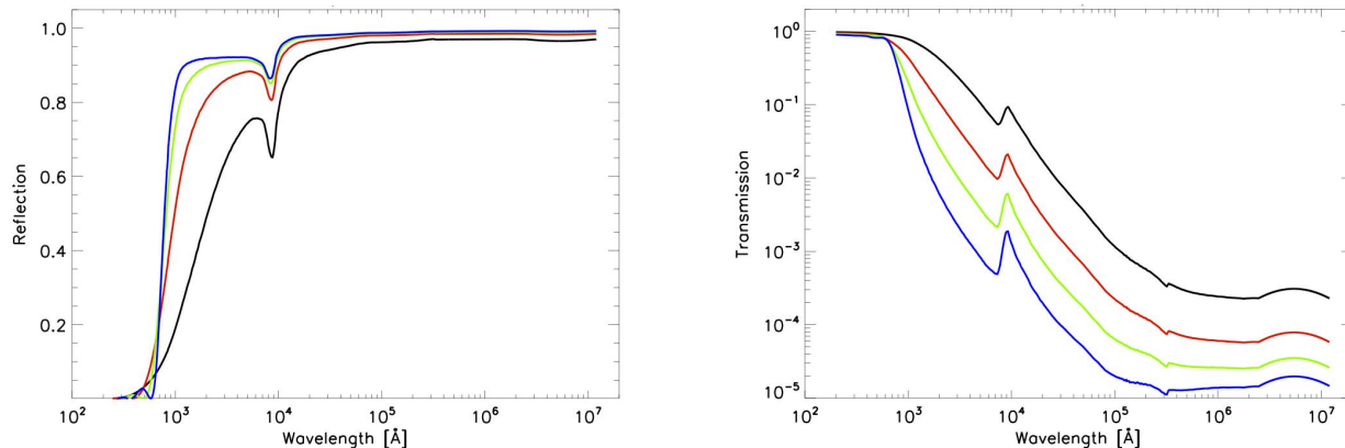
Figure 1. Calculated reflection of a single layer of aluminum 100 Å (black), 200 Å (red), 300 Å (green) and 400 Å thick (blue), respectively (left panel). Calculated transmission of the same layers of aluminum (right panel).
