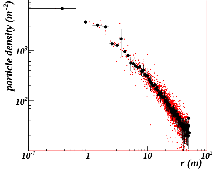
Figure 13: Lateral distribution of the particle density for the event shown in Fig.12. The red point are the measured density of particles on the BPs, while the black points are the mean values ( \pm r.m.s.) of the particle density measured in bins of distance, 0.5 m wide, from the shower core.
