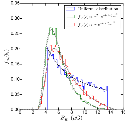
Figure A2. Distribution of the function B_R = B_0 e^{-r/r_B} for a uniform distribution of r given by U[R_{\min}, R_{\max}] (blue histogram) and for the case when r is distributed as per Eq. (7) with \eta = 1 (red histogram) and \eta = 2 (green histogram). The corresponding curves are the analytical PDFs given in Eqs. (A7) and (A8).
