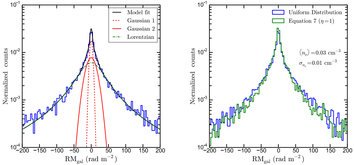
Figure 7. Left: Distribution of RM_{\text{gal}} for a sample of 10,000 galaxies with uniform distribution of i , \theta and r as described in Section 3.3 and, B_0 and n_0 of the sample have Gaussian distributions. The parameters used are listed in Table C1. The distribution is modelled as a sum of one Lorentzian and two Gaussian components and is shown as the black solid line. The individual components are shown as green dot-dashed, red solid and dashed lines. Right: Comparison of distribution of RM_{\text{gal}} when the radius at which the lines of sight intersect the galaxies are distributed uniformly same as left-hand panel (blue histogram) and for the case when they are distributed as in Eq. (7) with \eta = 1 (green histogram).
