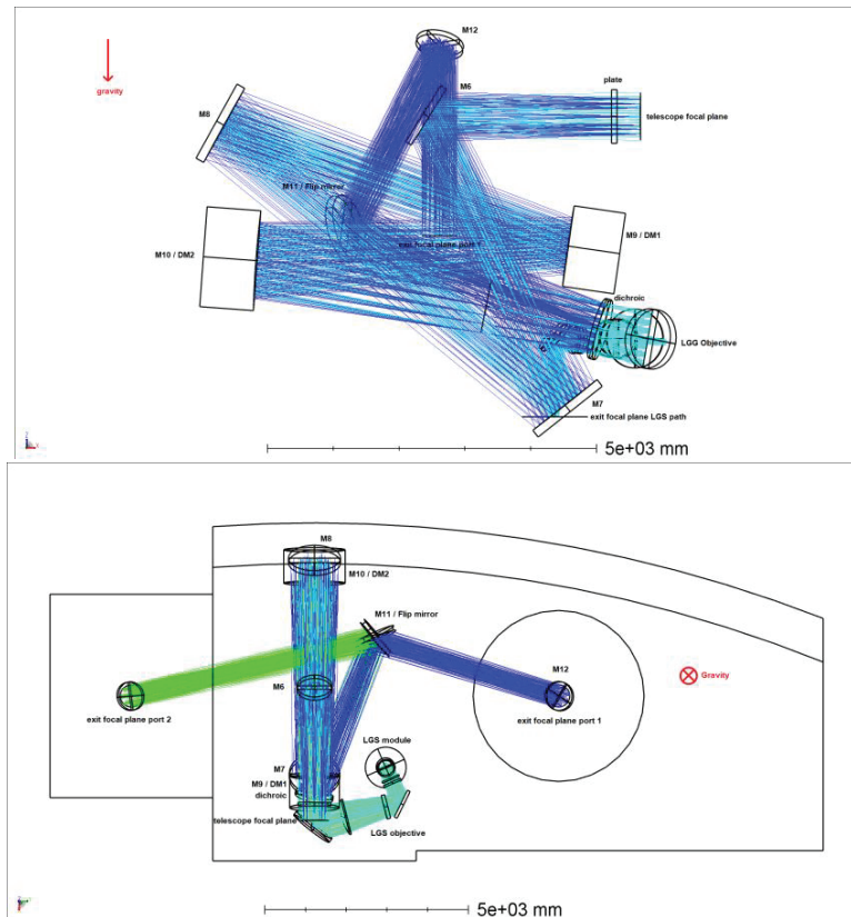
Figure 2 : Post-Focal Relay Optics baseline side way layout (top) and top view layout (bottom). Blue rays: optical beam from telescope focal plane to the exit port for MICADO. Green rays: differential path to exit port for second instrument. Light Blue rays: LGS path
