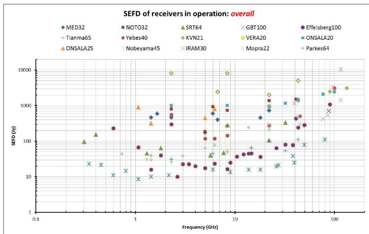
Figure 7.3 – SEFD for operational receivers
