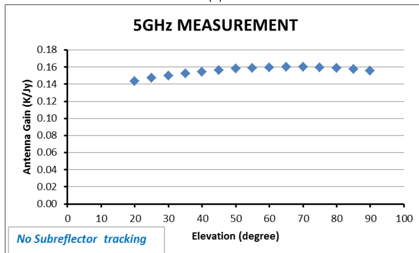
Figure D.2 – MED measured gain values at: (a) 22 GHz and (b) 5 GHz
