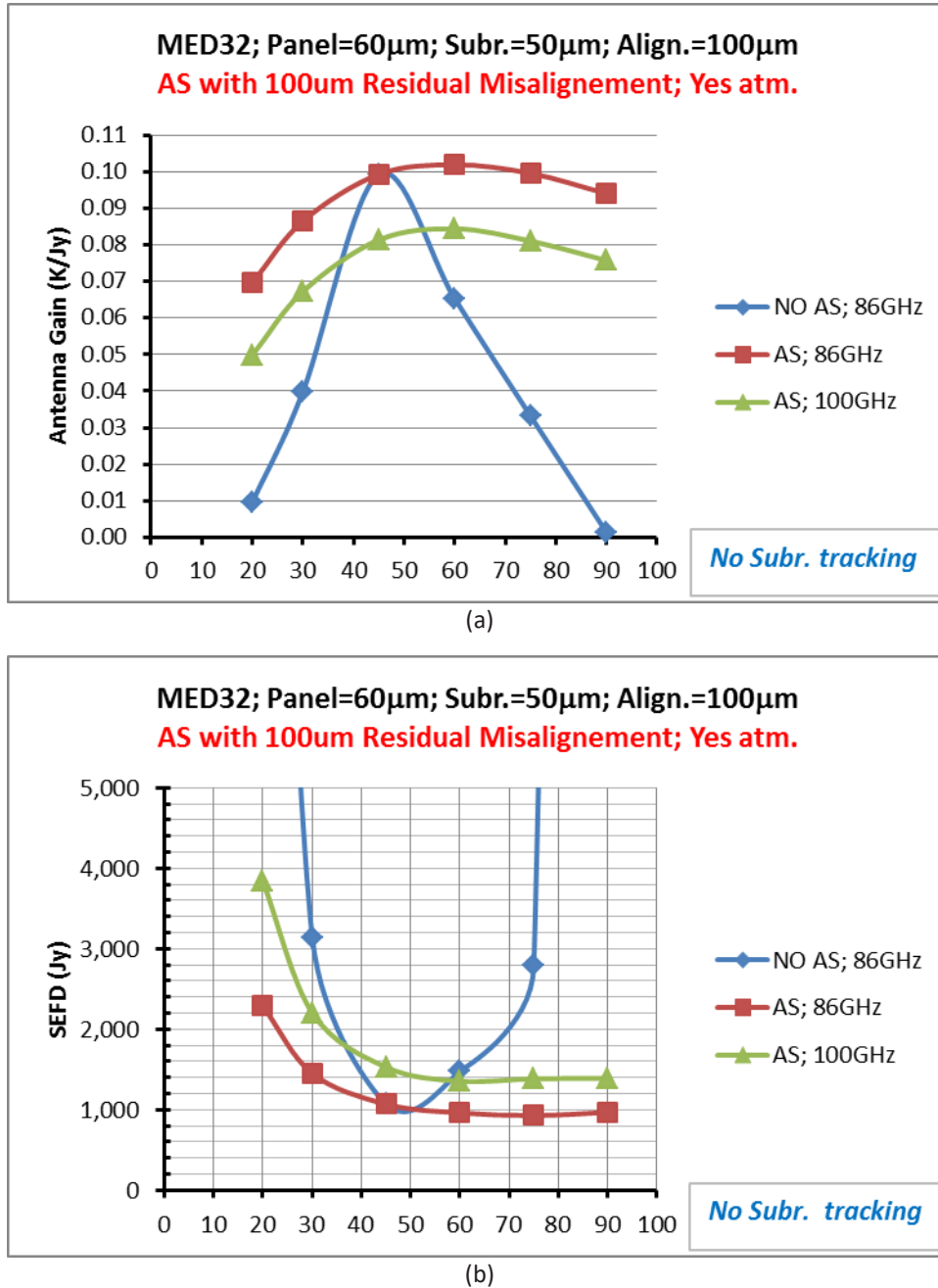
Figure D.5 – (a) Antenna gain and (b) SEFD, at 86 and 100 GHz including atmosphere effects. 86 GHz curves are given with and without active surface
