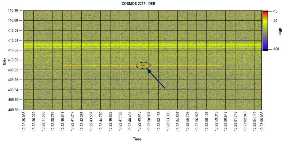
Figure 5.1 – Spectrogram of a space debris observation
