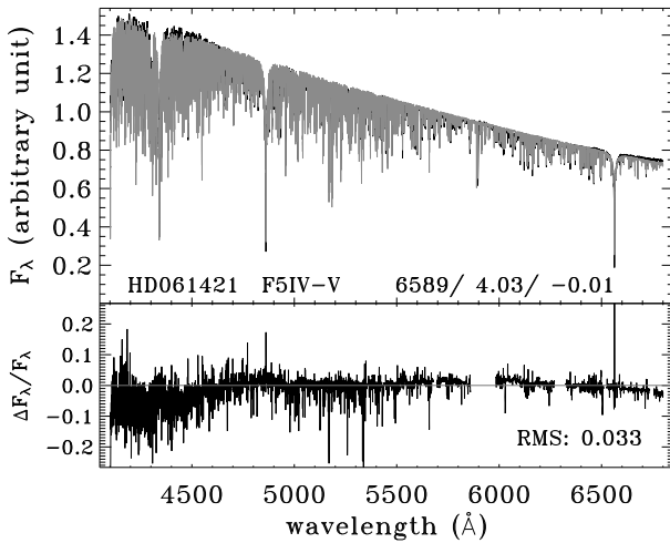
Fig. 9. ELODIE spectrum of HD 61421. In the upper panel, the SYNTH spectrum (grey line) is superimposed on the observed spectrum (black line). The relative flux residual is plotted in the lower panel.
