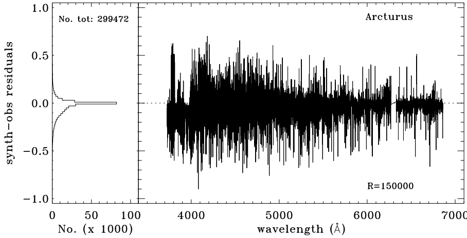
Fig. 5. Distribution of residual flux between the synthetic and observed spectrum of Arcturus. The observed SED is from Hinkle et al. (2000), at resolving power R \sim 150\,000 . BLUERED synthetic spectrum assumes (T_{\text{eff}}/\log g/[M/H]) = (4300/1.5/-0.5) (with some elemental overabundance, see Table 2). According to the definitions of Fig. 2, the systematic offset between observed and synthetic spectra amounts to \langle \Delta f_c/f_c \rangle = -0.037 , with a rms \sigma(r)_{\text{Arc}} = 0.108 and a skewness \gamma(r)_{\text{Arc}} = -0.67 .
